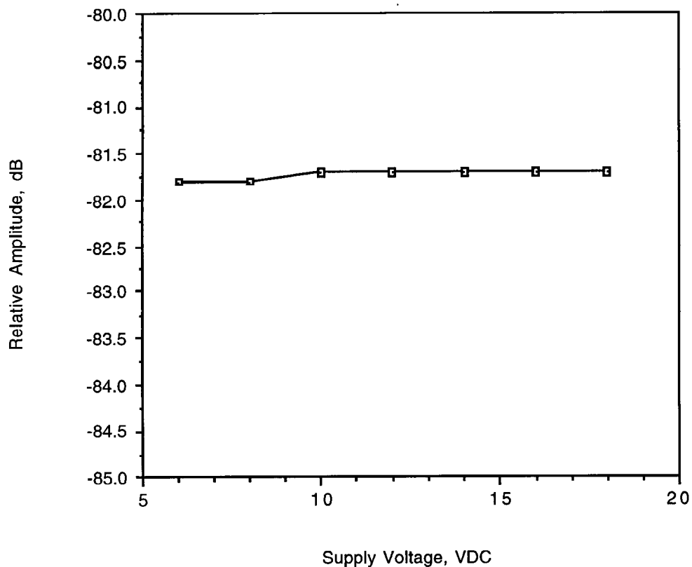
Figure 6.2. Relative emission at VCO (2xLO) vs. supply voltage.
