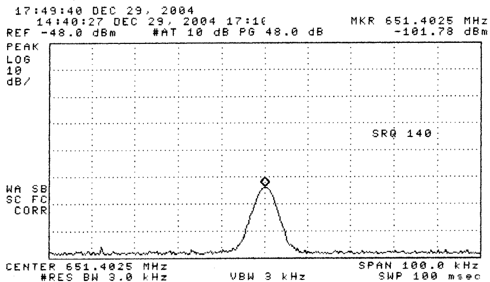
Figure 6.1. Receiver emission at VCO (2xLO). Conductive measurement.
