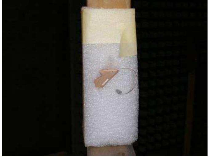
Img 4-5: Radiated emission - Electromagnetic field ( f \leq 1 GHz)
