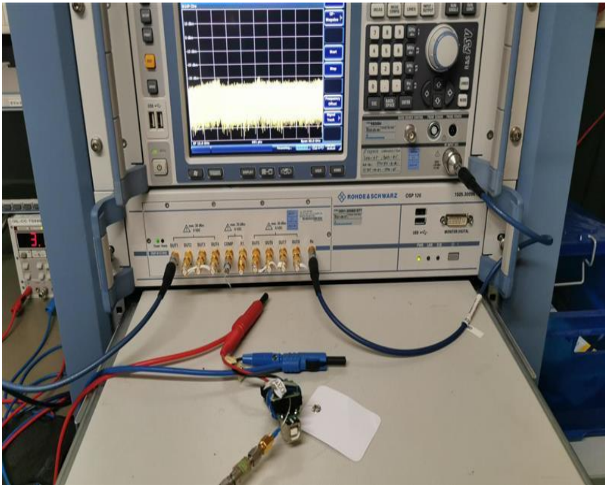
Photo 5: Test setup for conducted measurements on R&S TS8997
