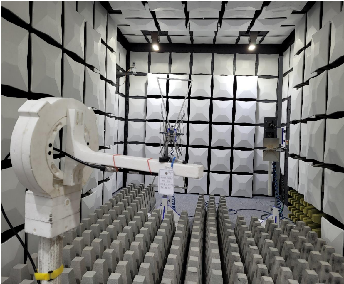
Photo 3: Test setup for radiated measurements (1 GHz – 26 GHz)
