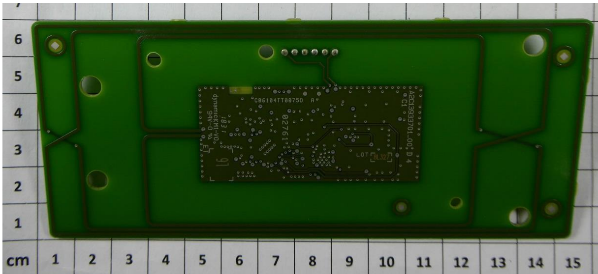
PCB mainboard – bottom view
