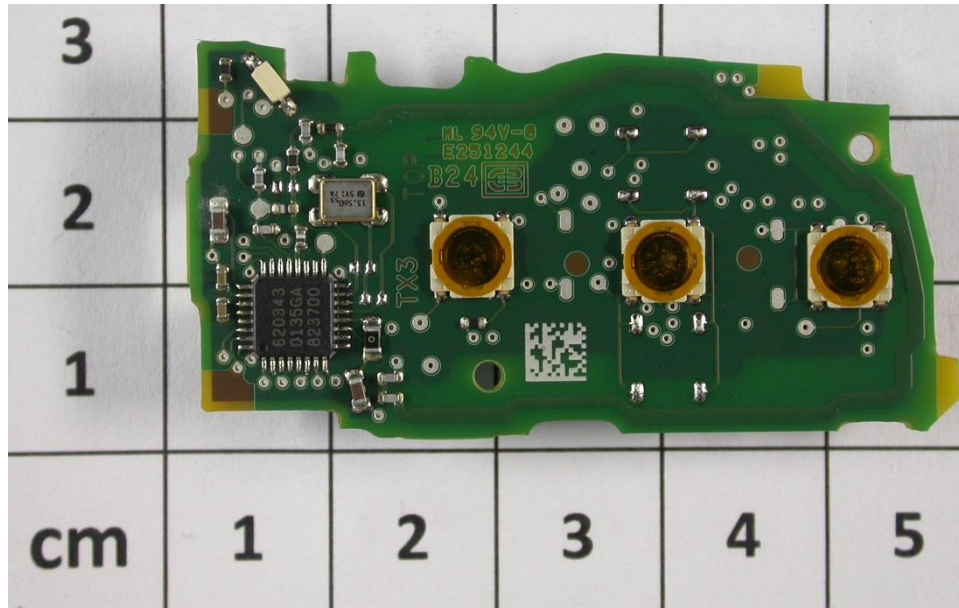
PCB mainboard – bottom view
