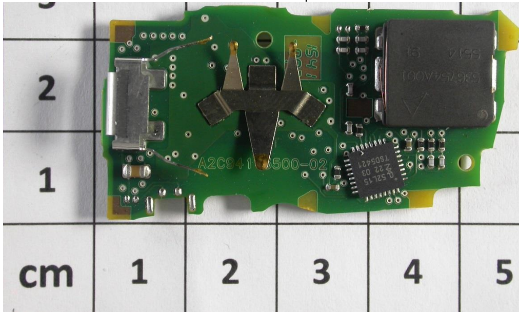
PCB mainboard – top view
