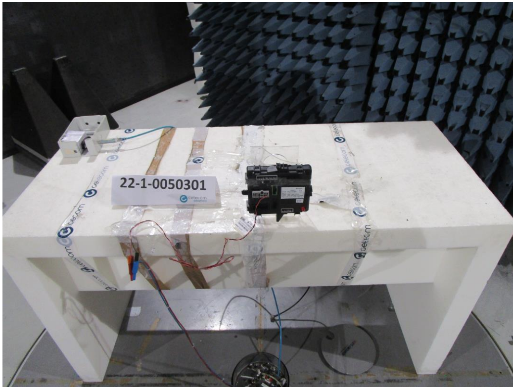
Fig. Mea.: 1 : Radiated Emission Radiated setup picture
