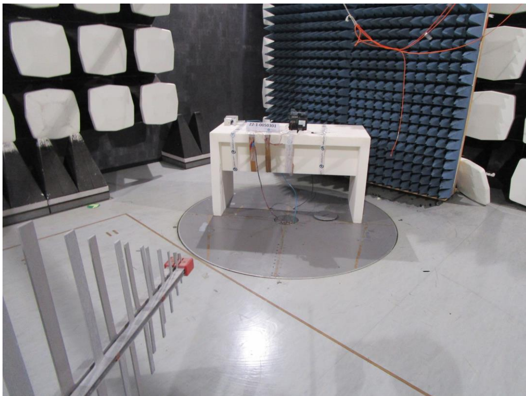
Fig. Mea.: 2 : Radiated Emission setup picture
