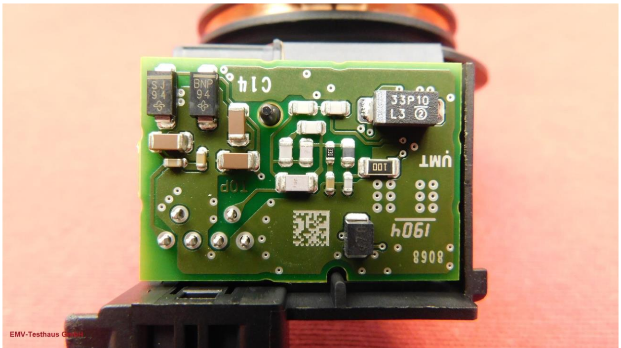
Picture 6: Bottom view of EUT with PCB
