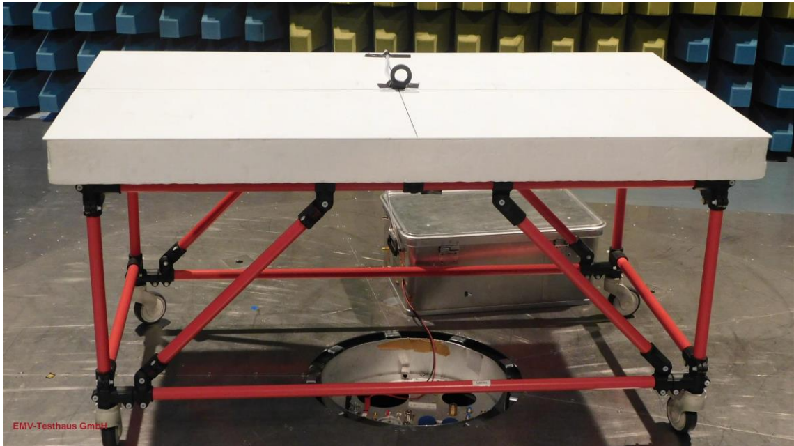
Picture 3: EUT test setup radiated emission test 30 MHz – 1 GHz (front view)
