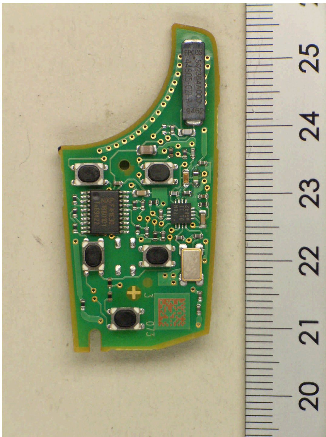
101797_12.jpg Global A Flap Key, PCB Matching N, top view
