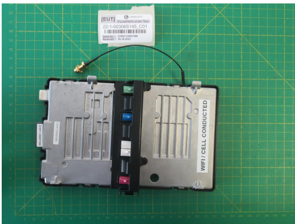
Fig. Ext.: 6 : Ext. - Rear Telematic Control Unit EUT 3
