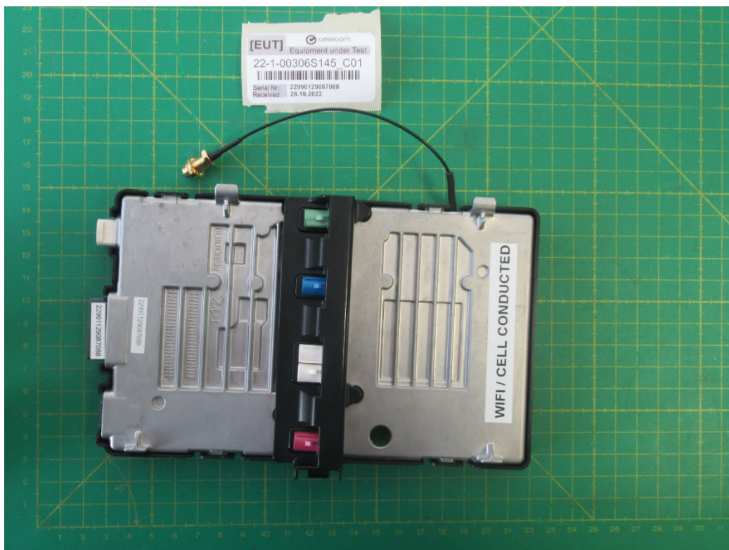
Fig. Ext.: 4 : Ext. - Rear Telematic Control Unit EUT 2
