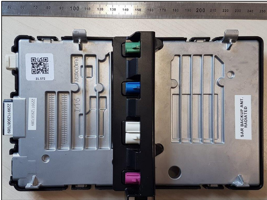
Photo 4: Test position front side with 15 mm distance
