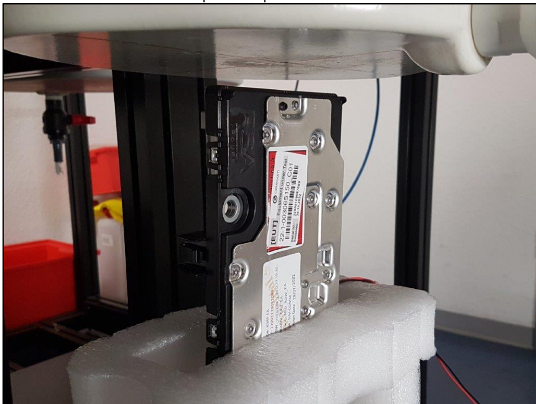
Photo 7: Test position top side with 15 mm distance
