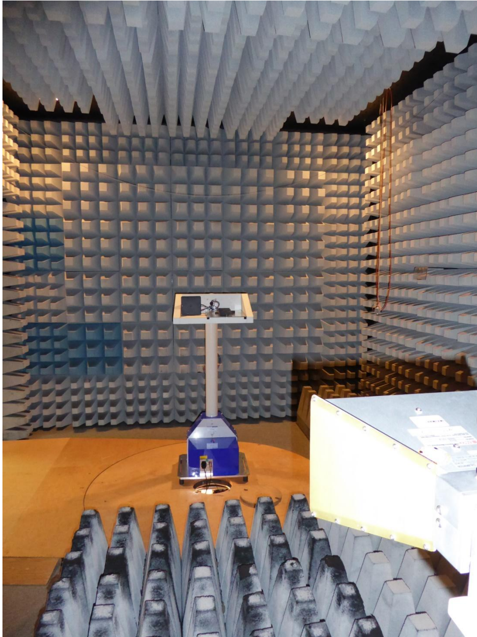
154295_22.JPG: Test setup fully anechoic chamber (1 GHz to 5 GHz)
