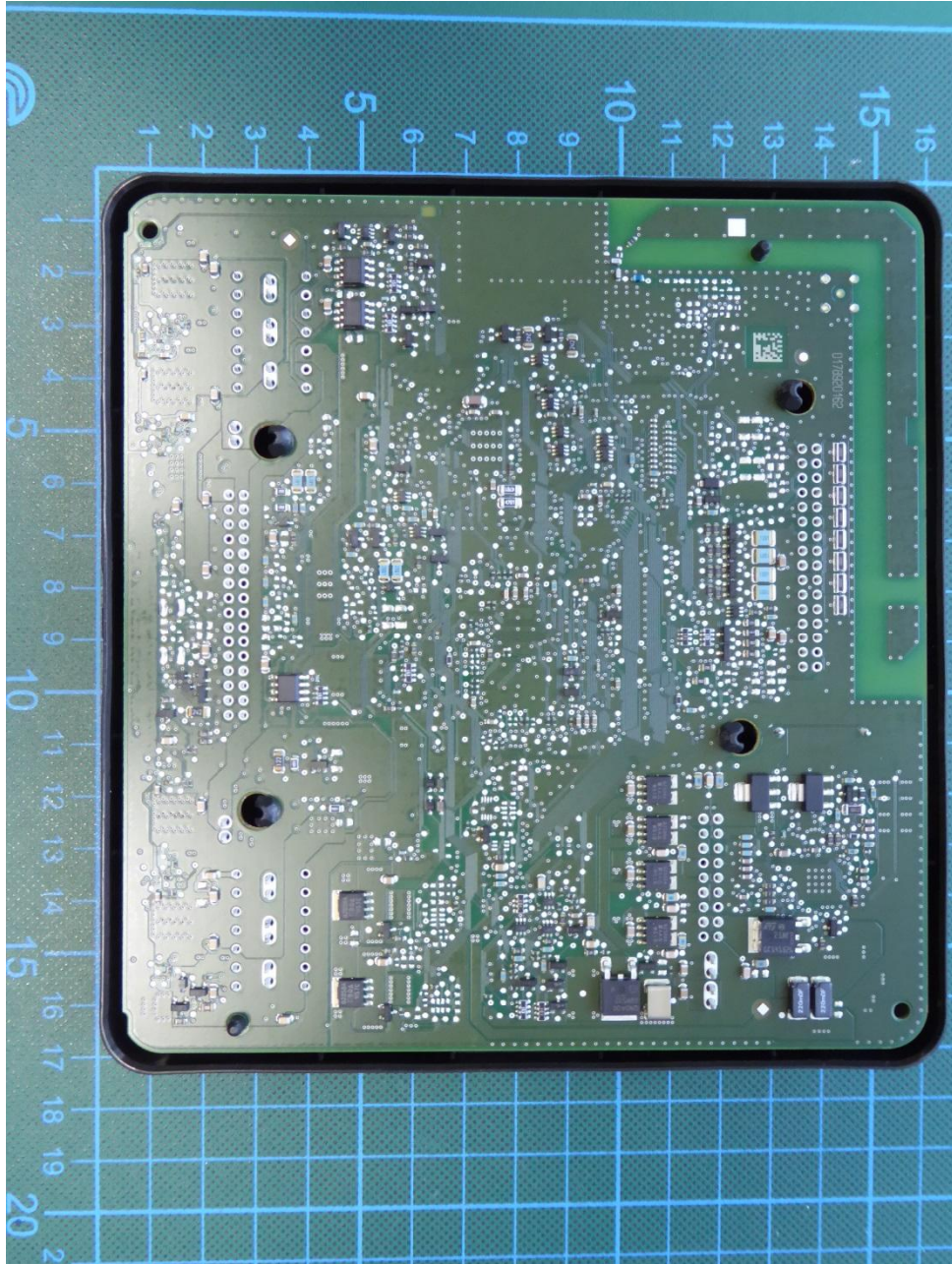
154295_5.JPG: PCB, top view
