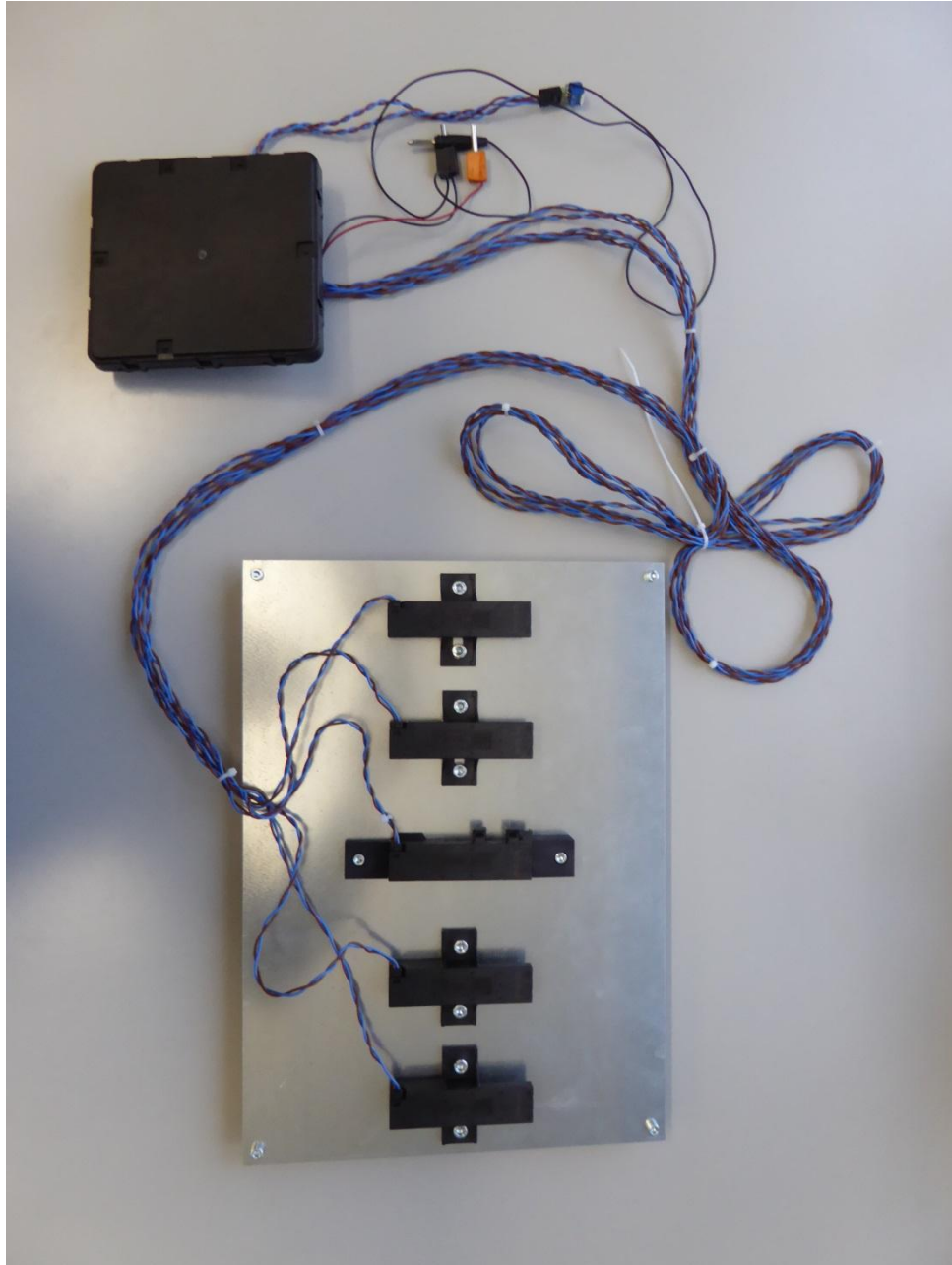
154295_1.JPG: EUT with LF antennas and harness
