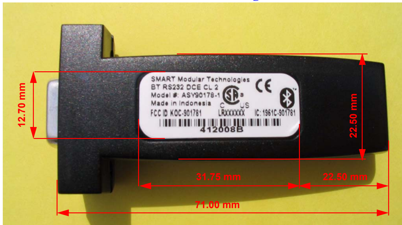
Bottom View - Bluetooth RS232 DCE Class 2, Model ASY90178-1
