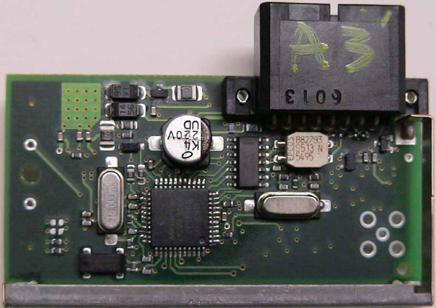
PCB (top)
