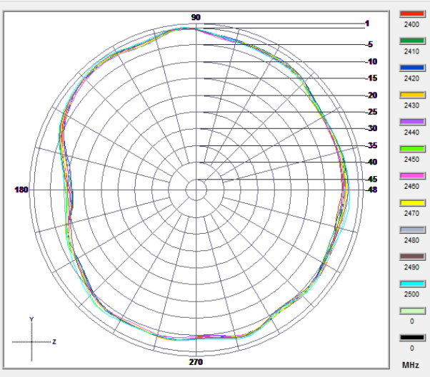
YZ
