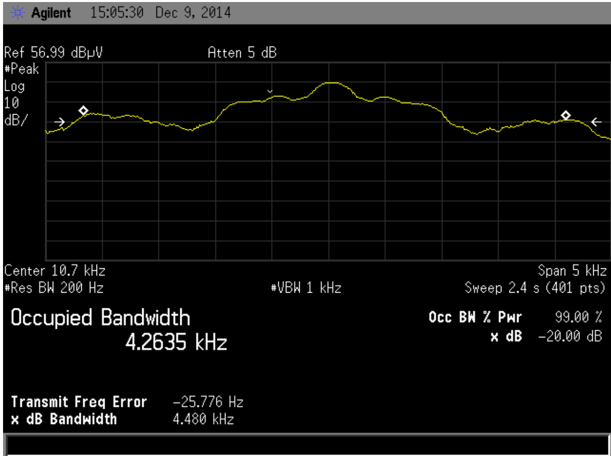
Figure 2. 20 dB & 99% Bandwidth
