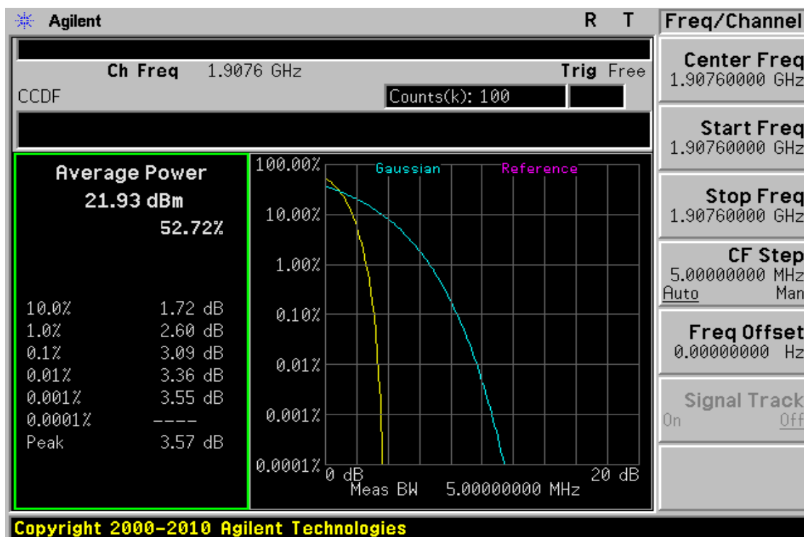
Figure 7-21: WCDMA Band II Channel High
