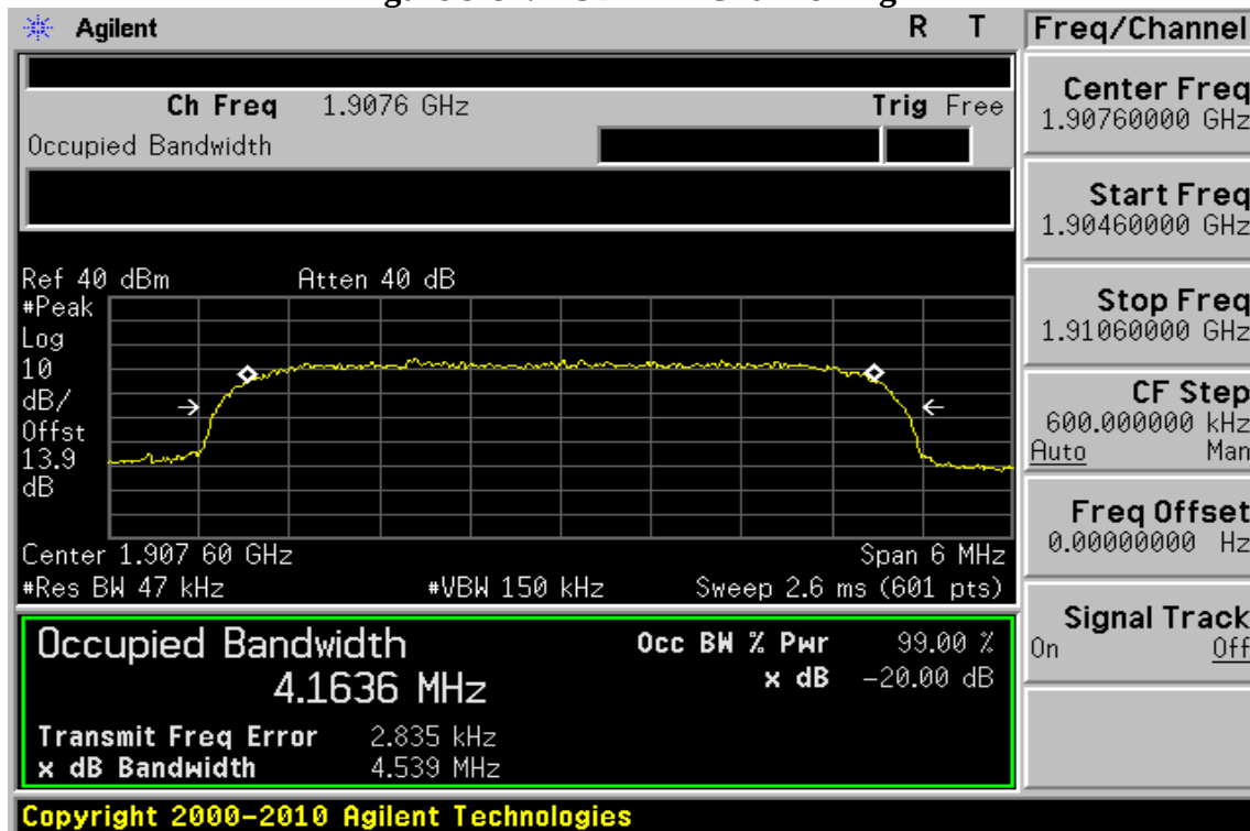
Figure 9-84: HSDPA II Channel High
