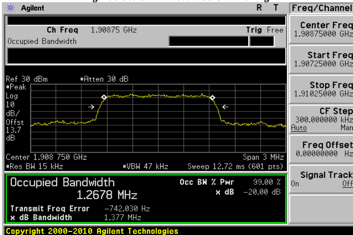
Figure 9-96: CDMA 2000 PCS Channel High
