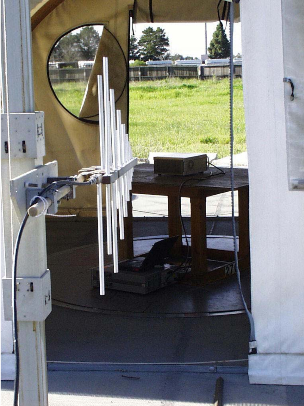
Radiated emissions test setup, LPA antenna
