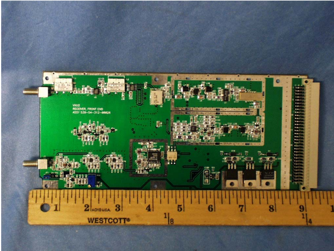
Receiver board top no cans
