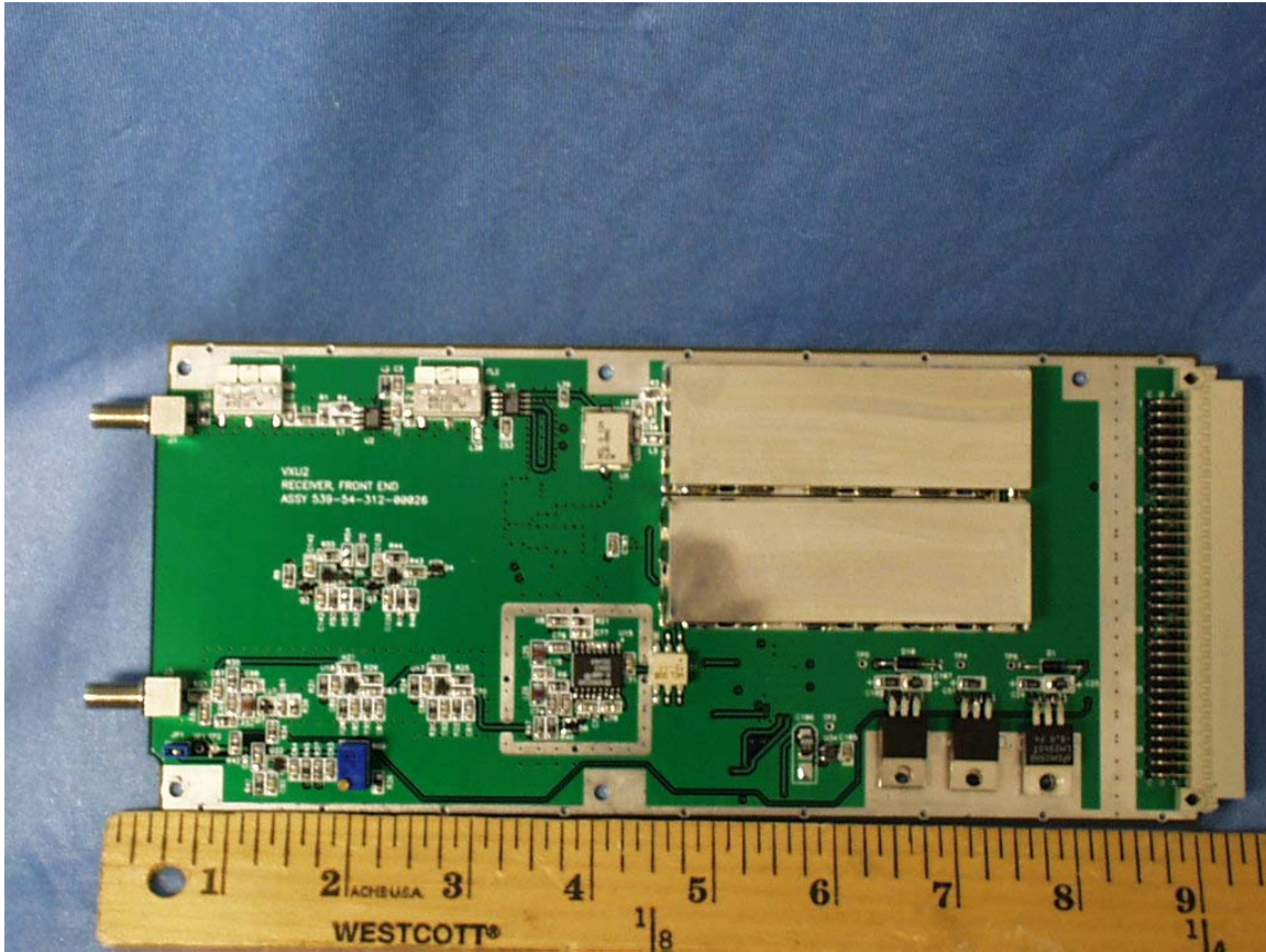
Receiver board top
