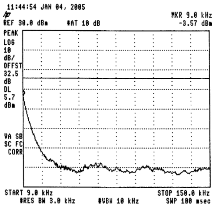
Figure 37 —915.0 MHz
