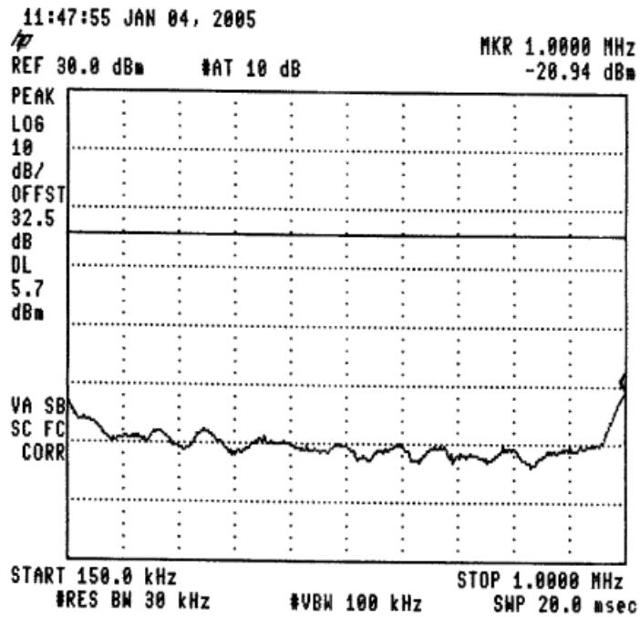
Figure 38 —915.0 MHz
