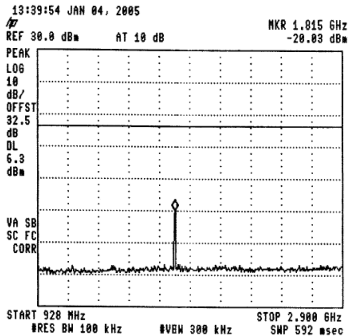
Figure 33 —904.6 MHz
