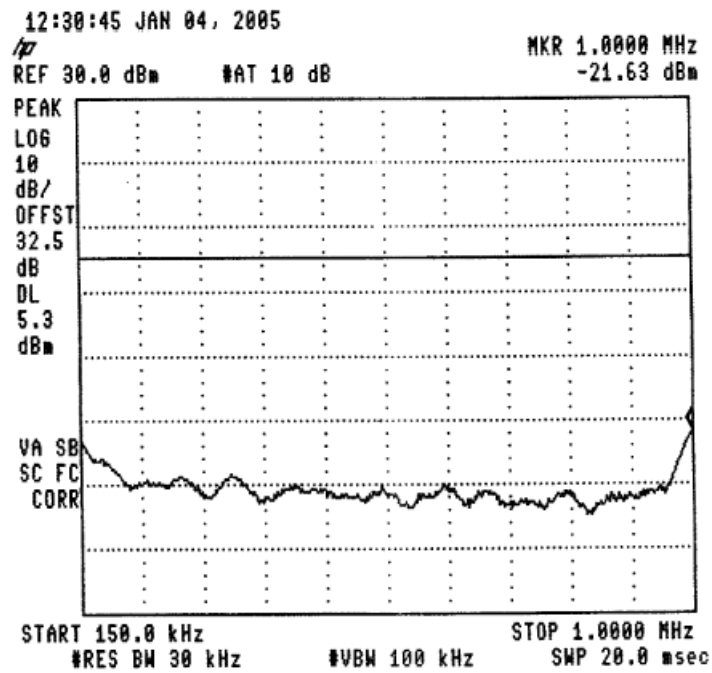
Figure 46 —925.4 MHz
