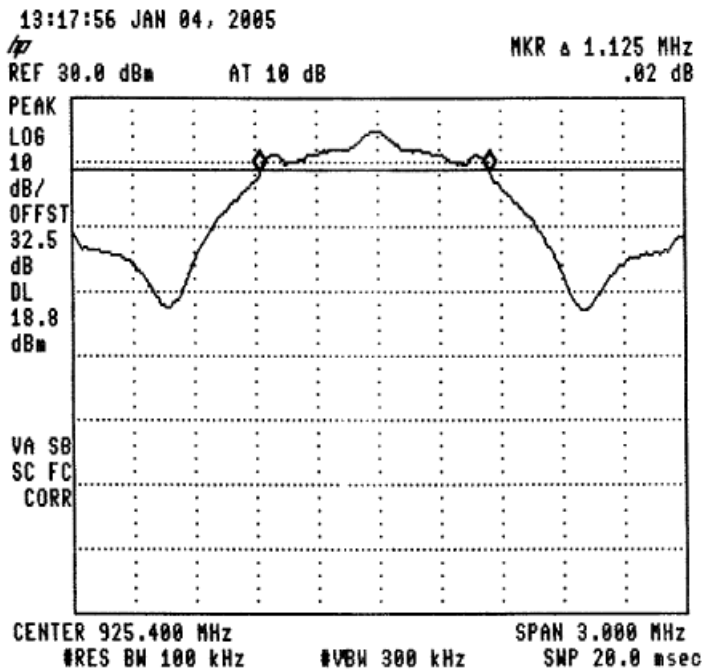
Figure 57 —925.4 MHz
