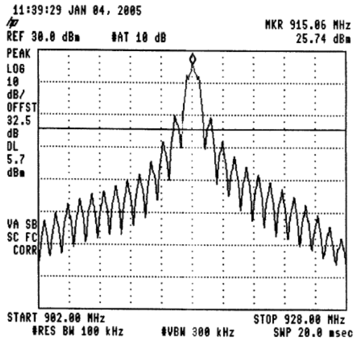
Figure 36 —915.0 MHz
