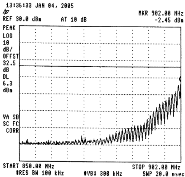
Figure 32 —904.6 MHz
