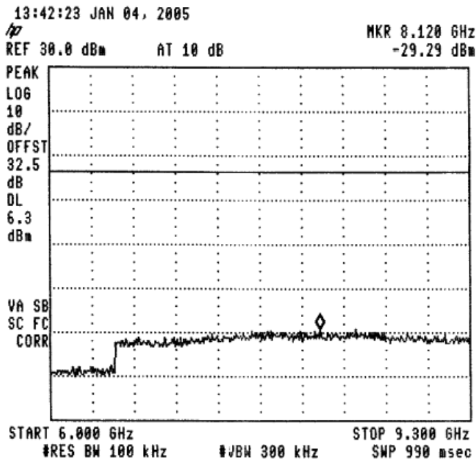
Figure 35 —904.6 MHz
