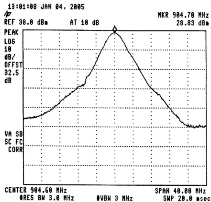
Figure 22 904.6 MHz
