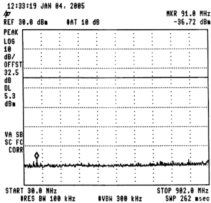
Figure 48 —925.4 MHz
