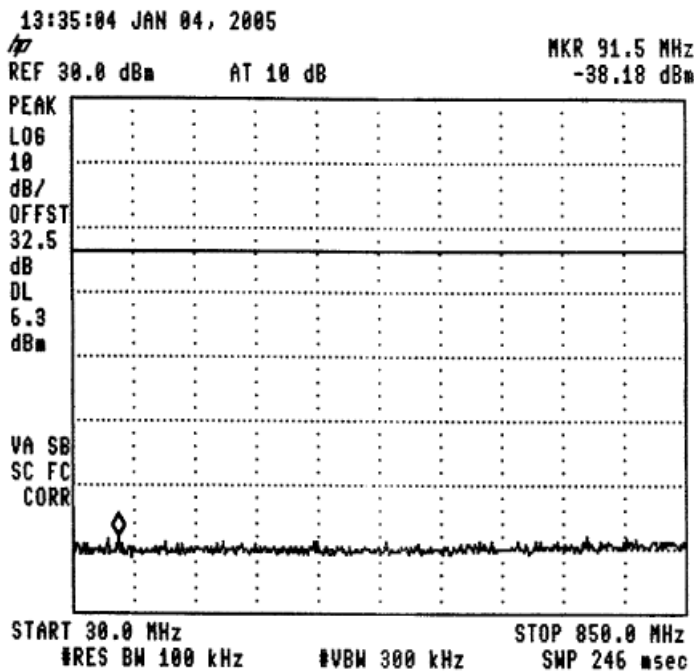
Figure 31 —904.6 MHz
