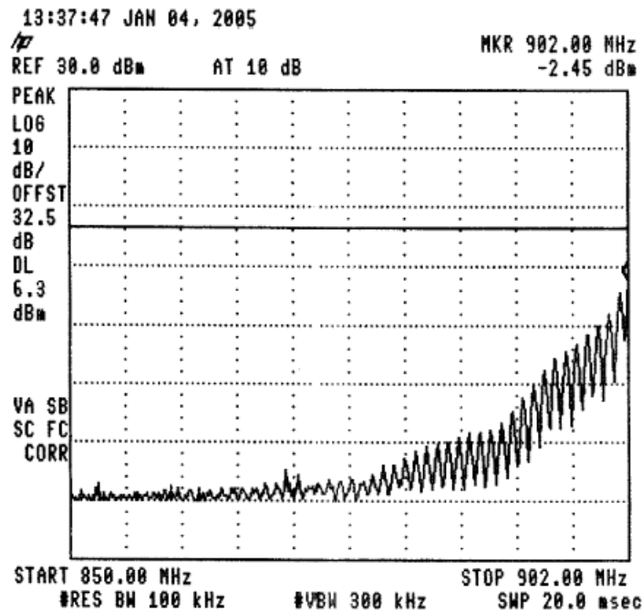
Figure 60 —904.6 MHz
