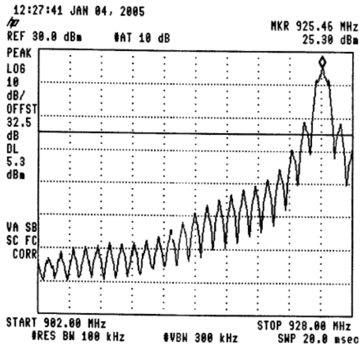
Figure 44 —925.4 MHz
