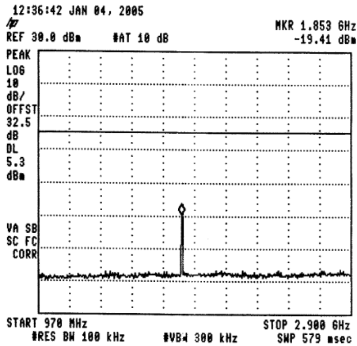
Figure 50 —925.4 MHz
