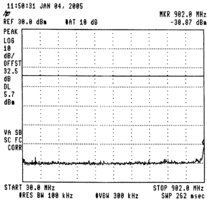
Figure 40 —915.0 MHz
