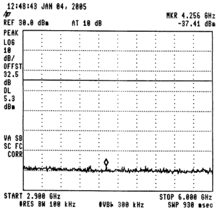
Figure 51 —925.4 MHz
