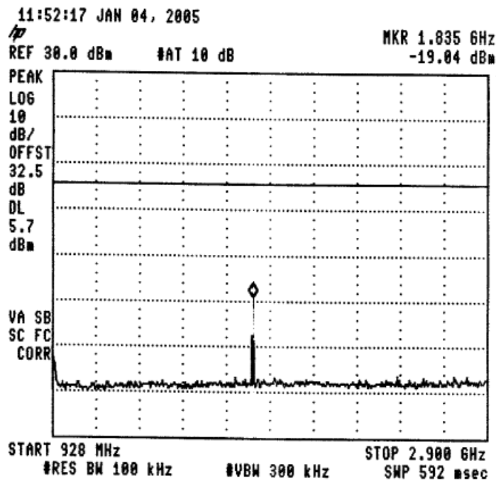
Figure 41 —915.0 MHz
