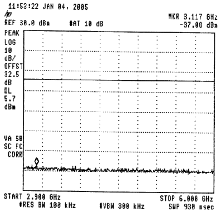
Figure 42 —915.0 MHz
