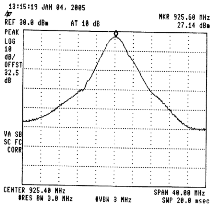
Figure 24 925.4 MHz
