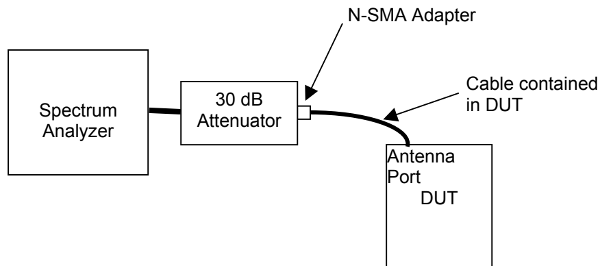
Figure C.6-1 - Setup Drawing
