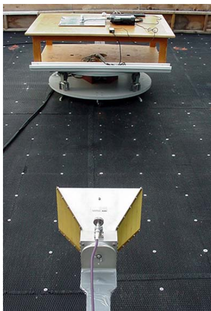
Photograph J.7-4 - Mobile - 3 m Horn Setup
