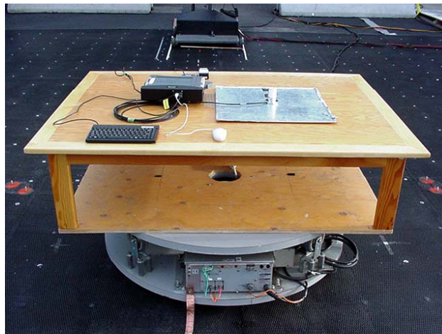
Photograph J.7-2 - Mobile DUT Configuration
