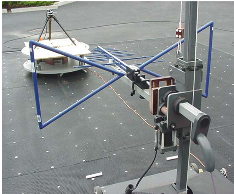
Substitution Dipole antenna and Bilog receive antenna
