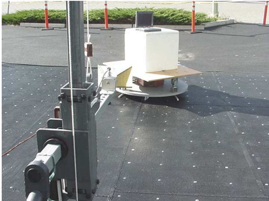
DUT PCS Band with Horn receive antenna
