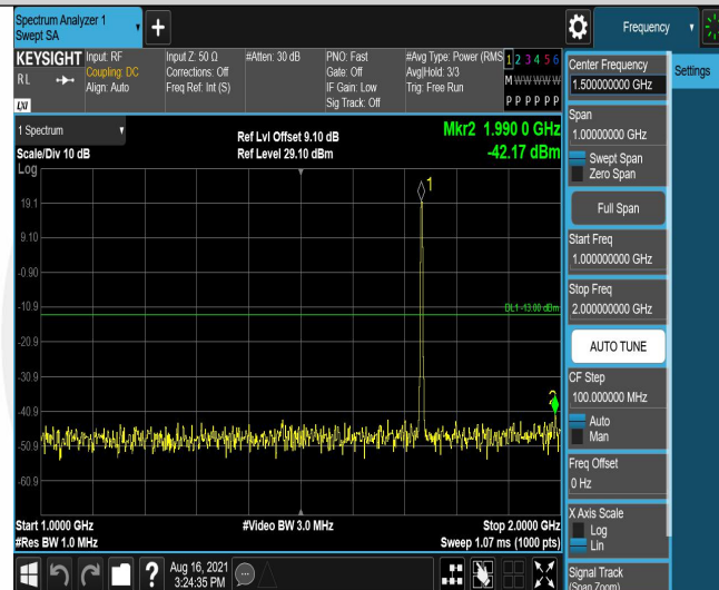
Band4-1.4MHz-16QAM-20175-6RB#0-Range2:1000~2000MHz
