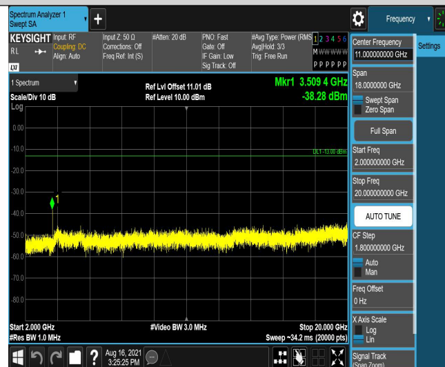
Band4-1.4MHz-QPSK-20393-6RB#0-Range3:2000~20000MHz
