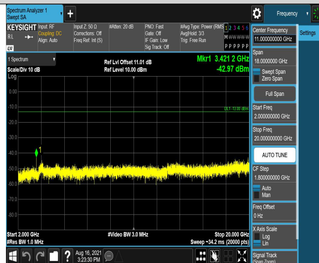
Band4-1.4MHz-16QAM-19957-6RB#0-Range3:2000~20000MHz
