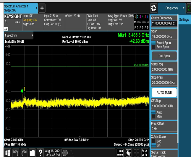
Band4-1.4MHz-16QAM-20175-6RB#0-Range3:2000~20000MHz
