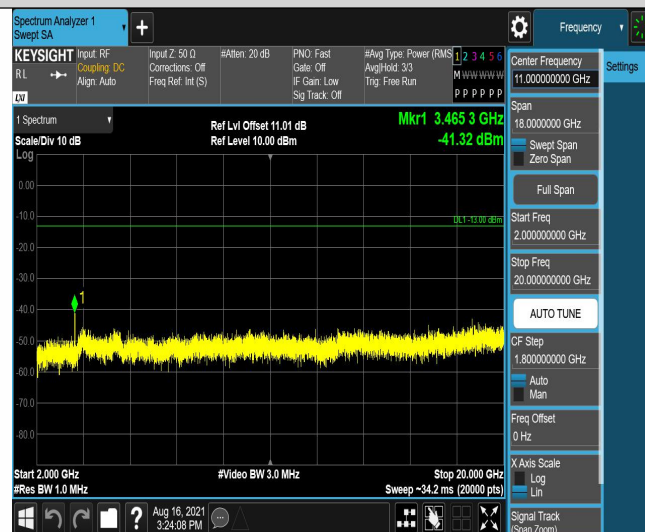
Band4-1.4MHz-QPSK-20175-6RB#0-Range3:2000~20000MHz
