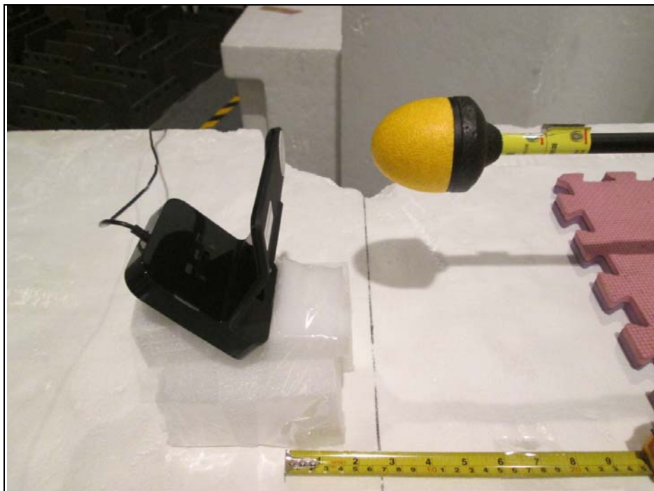
E-Field (Z-axis) (Standby Mode)
