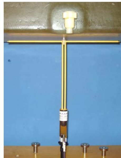
SPEAG 300 MHz Validation Dipole Setup
