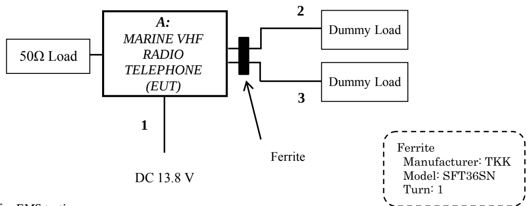
Setup diagram for EMS testing
