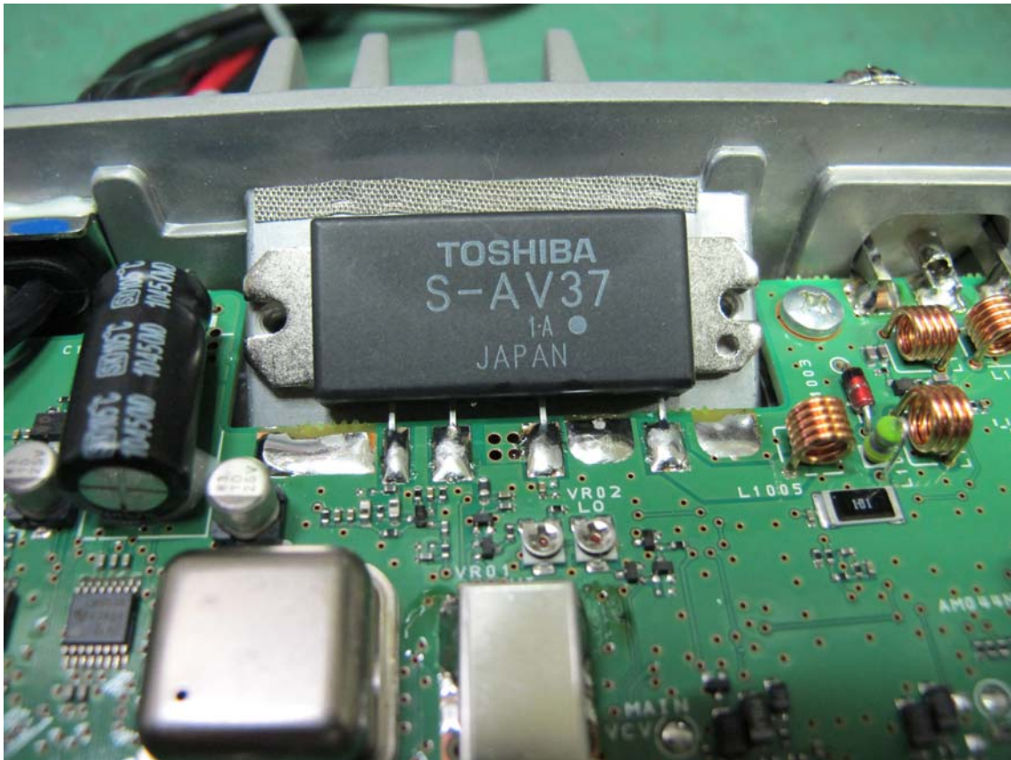
Original Power Module without Shield cover
