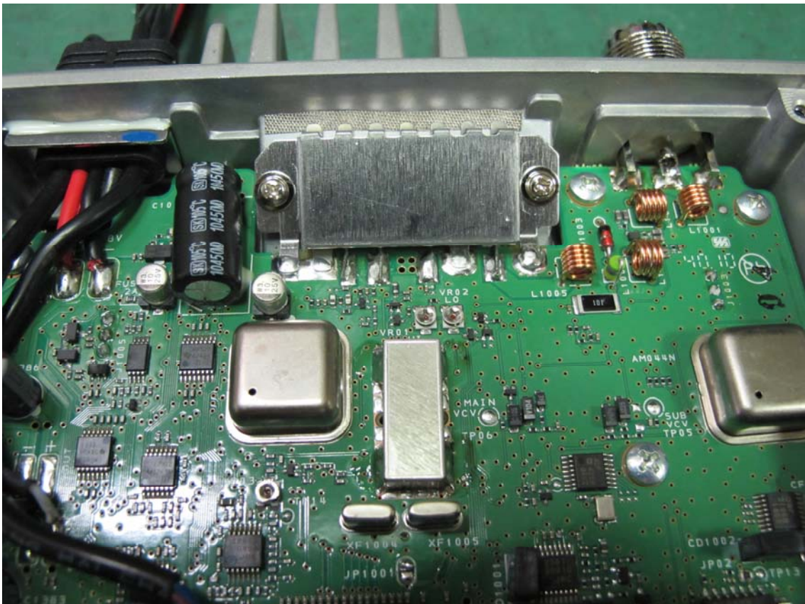
Replacement Power Module with Shield cover
