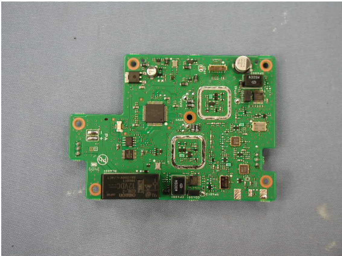
Side-A of AIS-UNIT without shield cases (GX2100)
