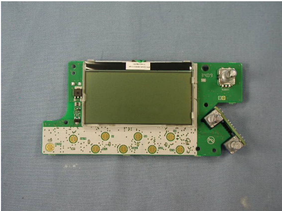
Side-A of CNTL-UNIT with LCD and VR-UNIT
