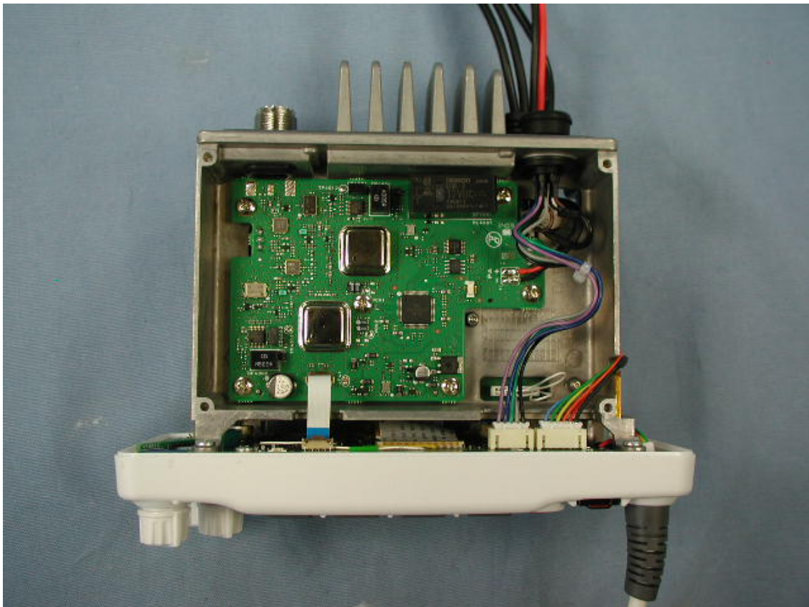
Bottom of EUT without case (GX2100)
