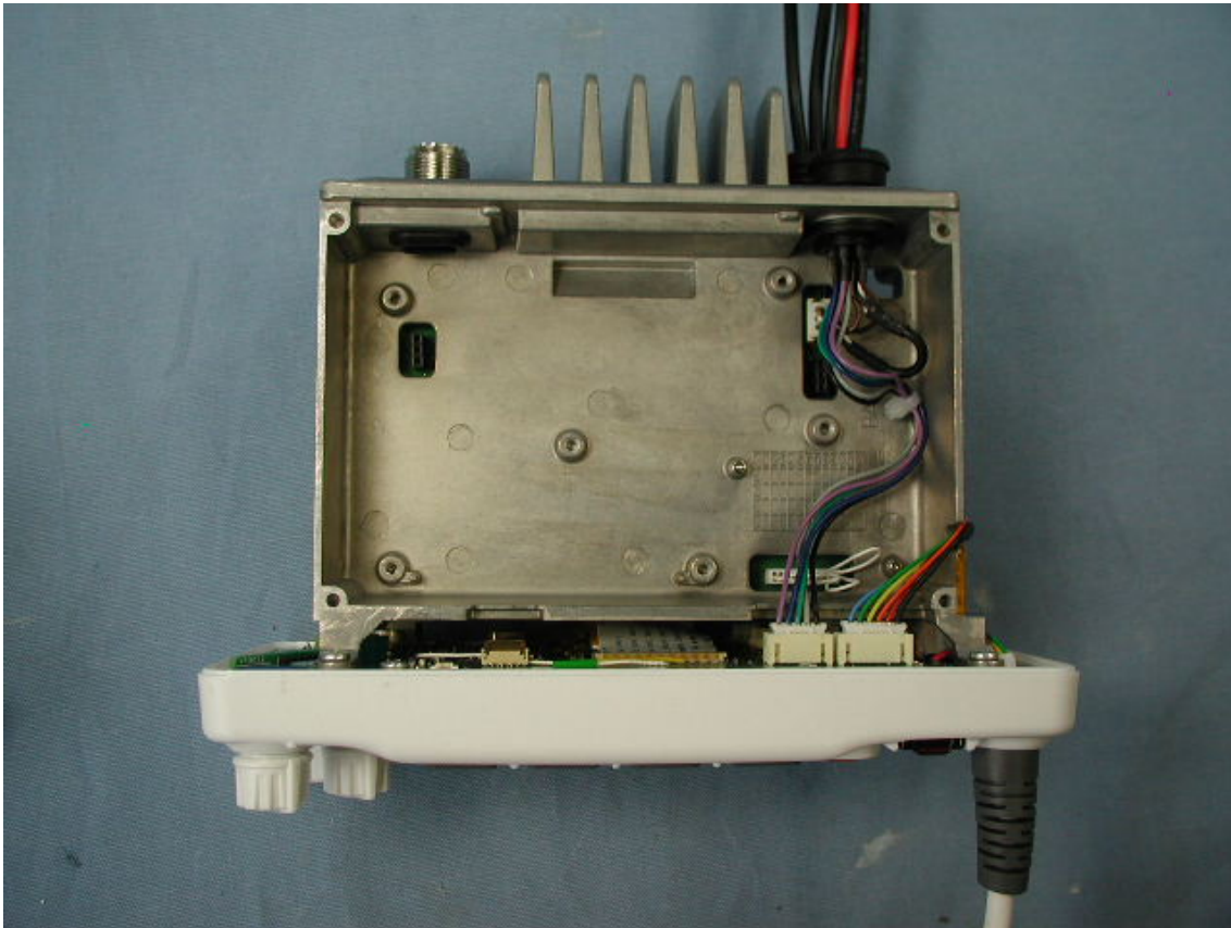
Bottom of EUT without case (GX2000)
