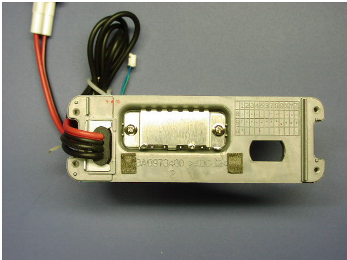
Replacement Power Module with Shield case
