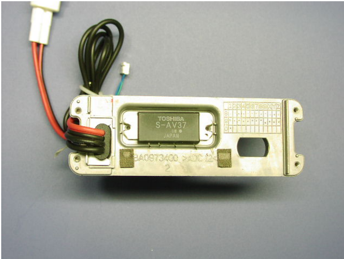
Original Power Module without Shield case
