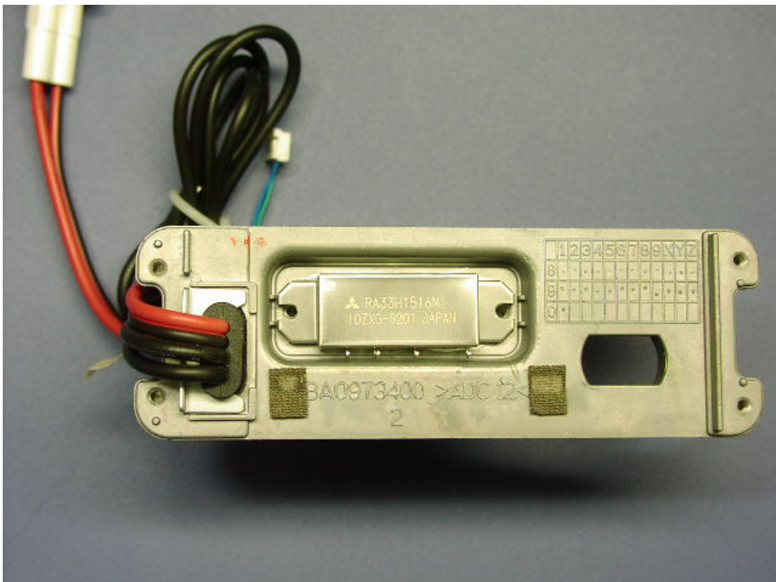
Replacement Power Module without Shield case
