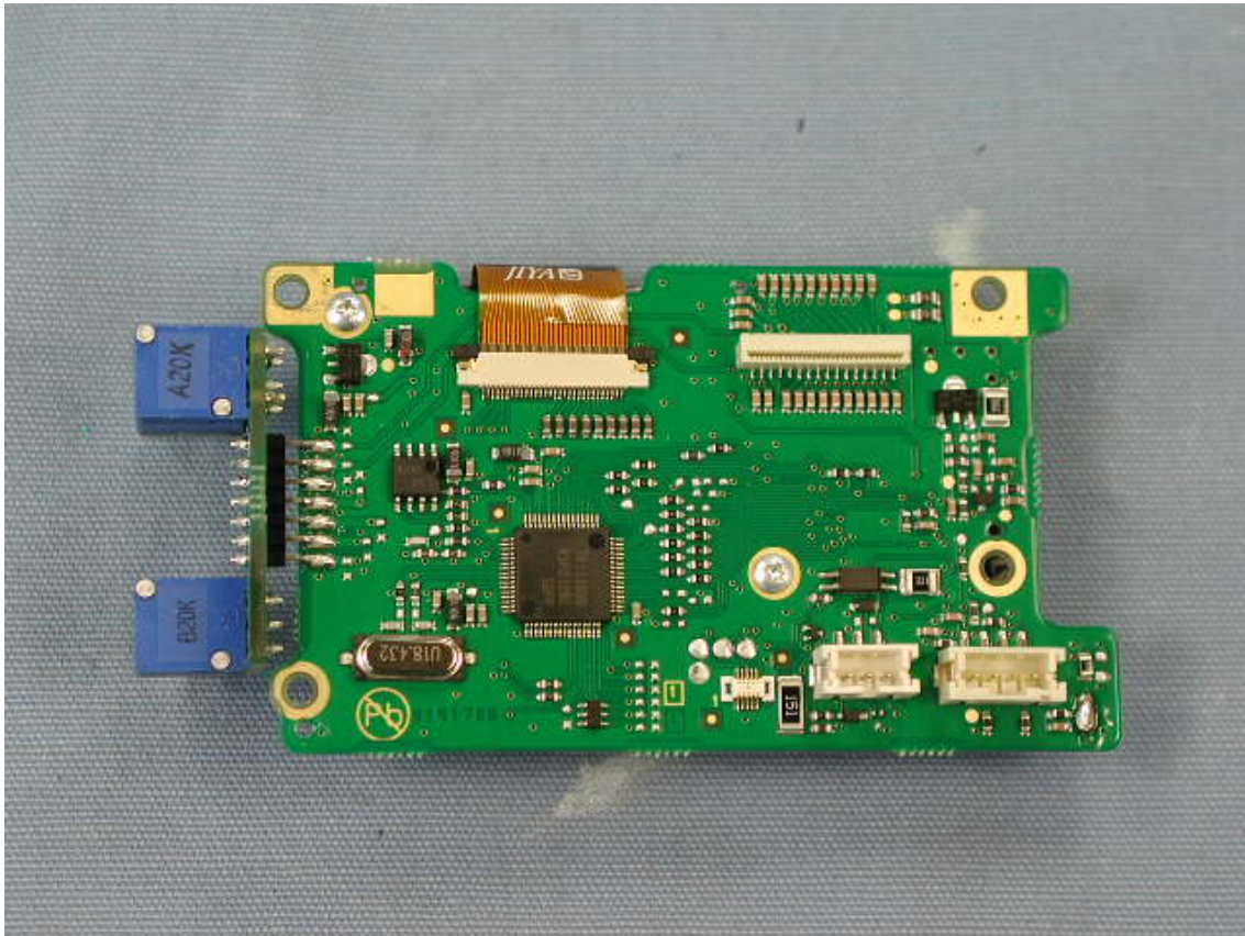
Side-B of CNTL-UNIT and VR-UNIT
