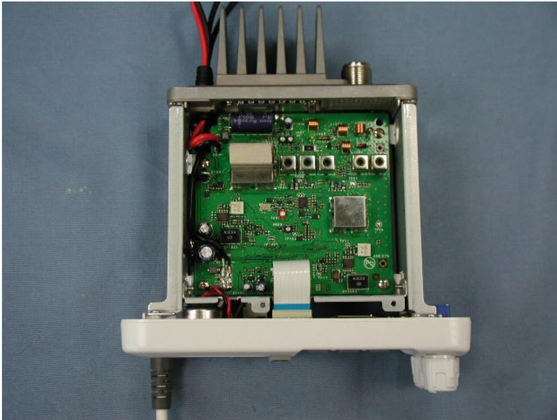
Top of EUT without shield
