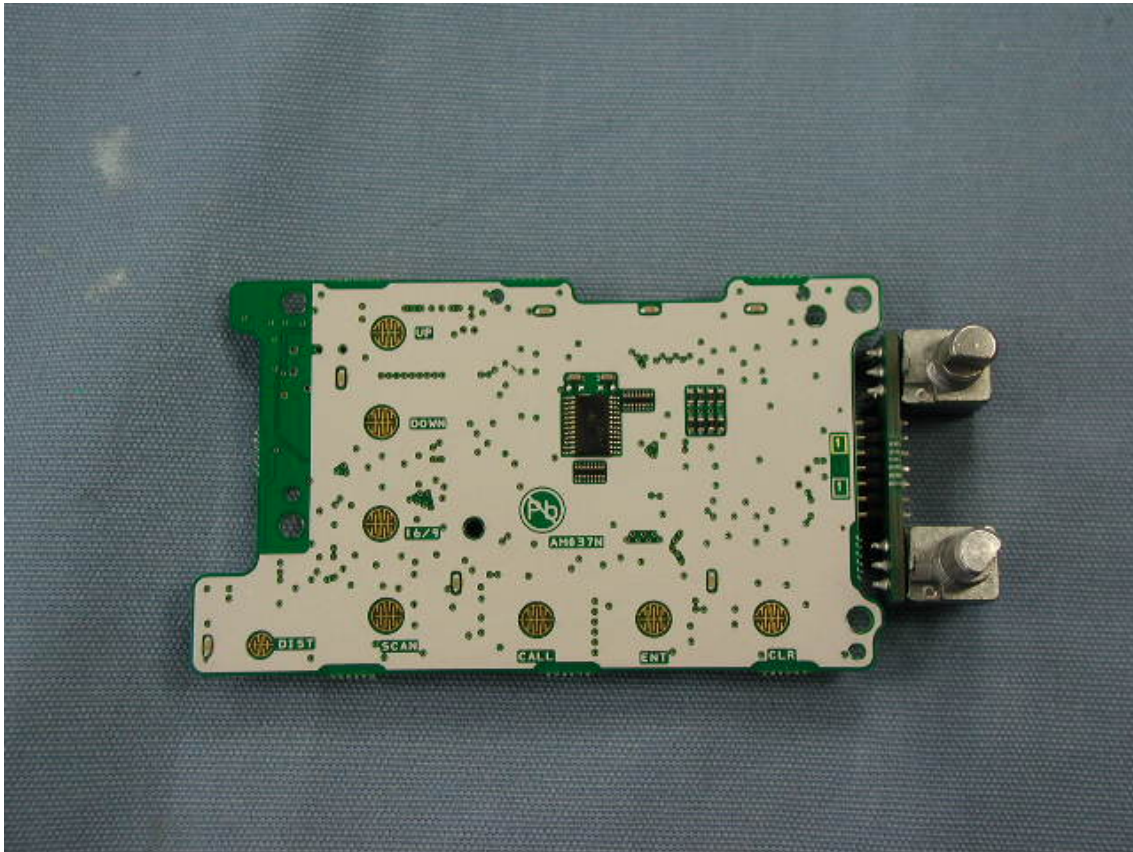
Side-A of CNTL-UNIT and VR-UNIT without LCD
