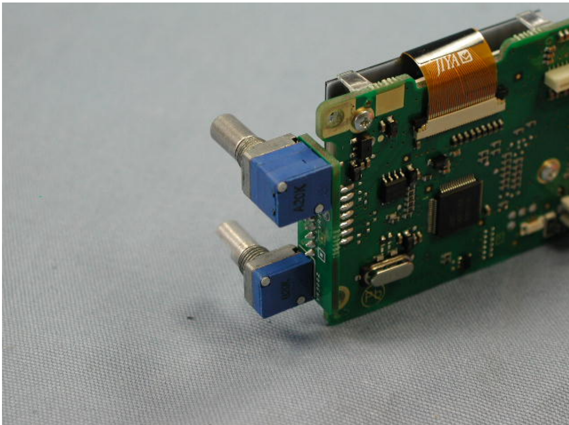
View of VR-UNIT
