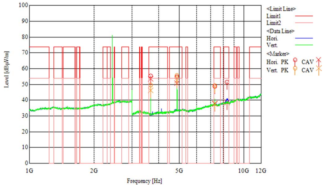
[Chart] TX 2440MHz DH5 Y-plane
