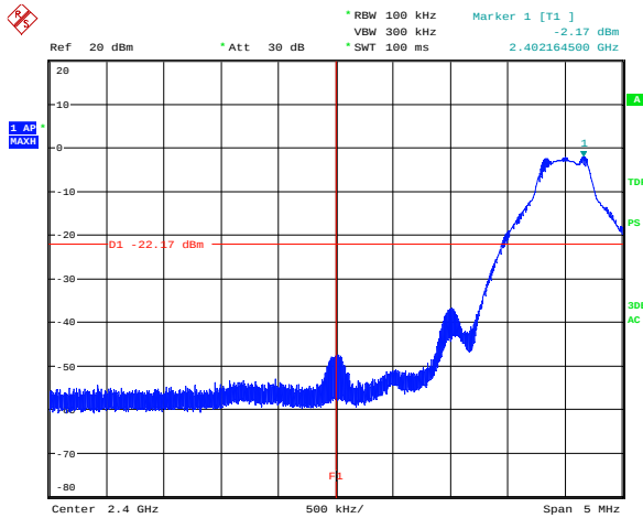
Tx 2402 MHz DH5
