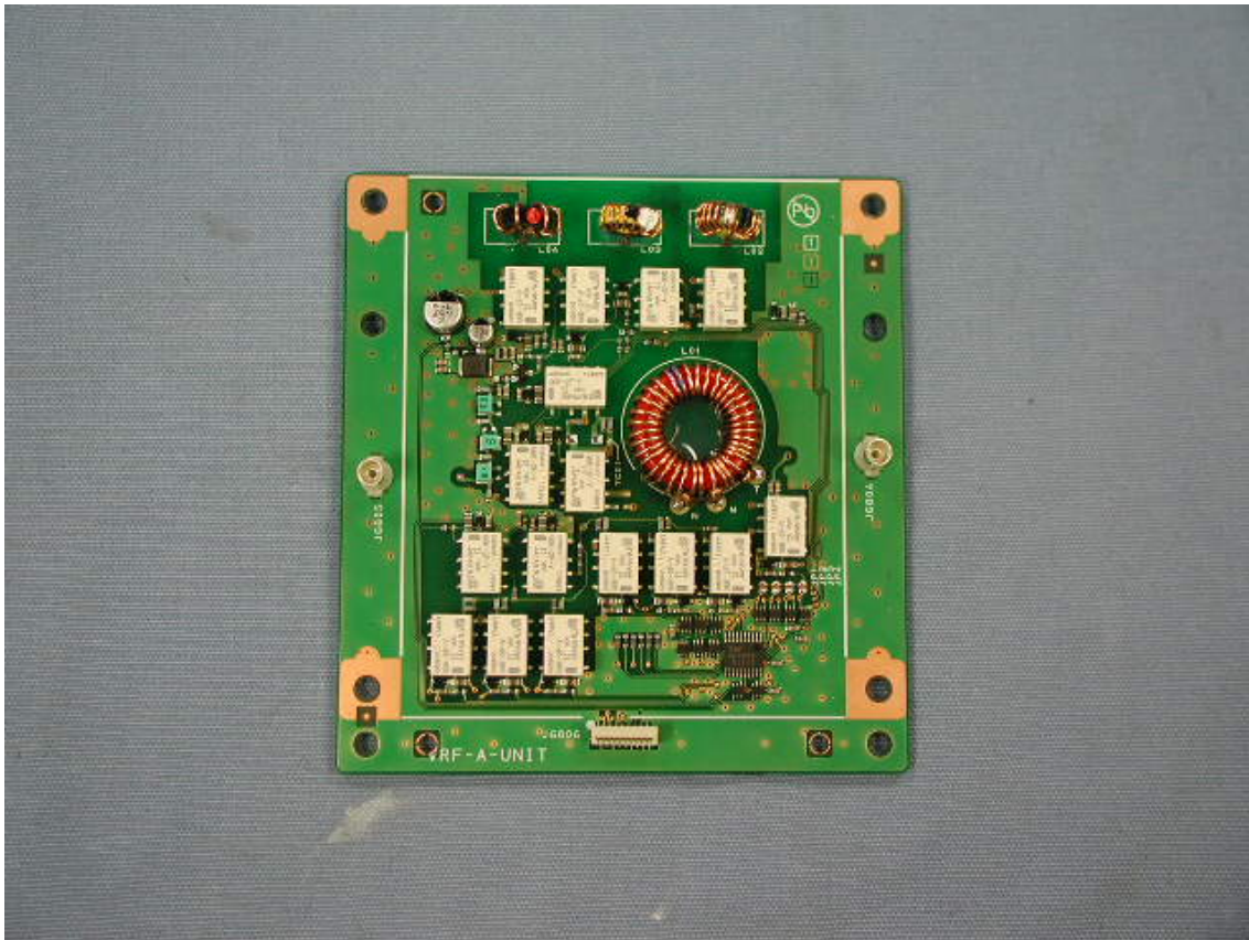
Side-A of VRF-A-UNIT
