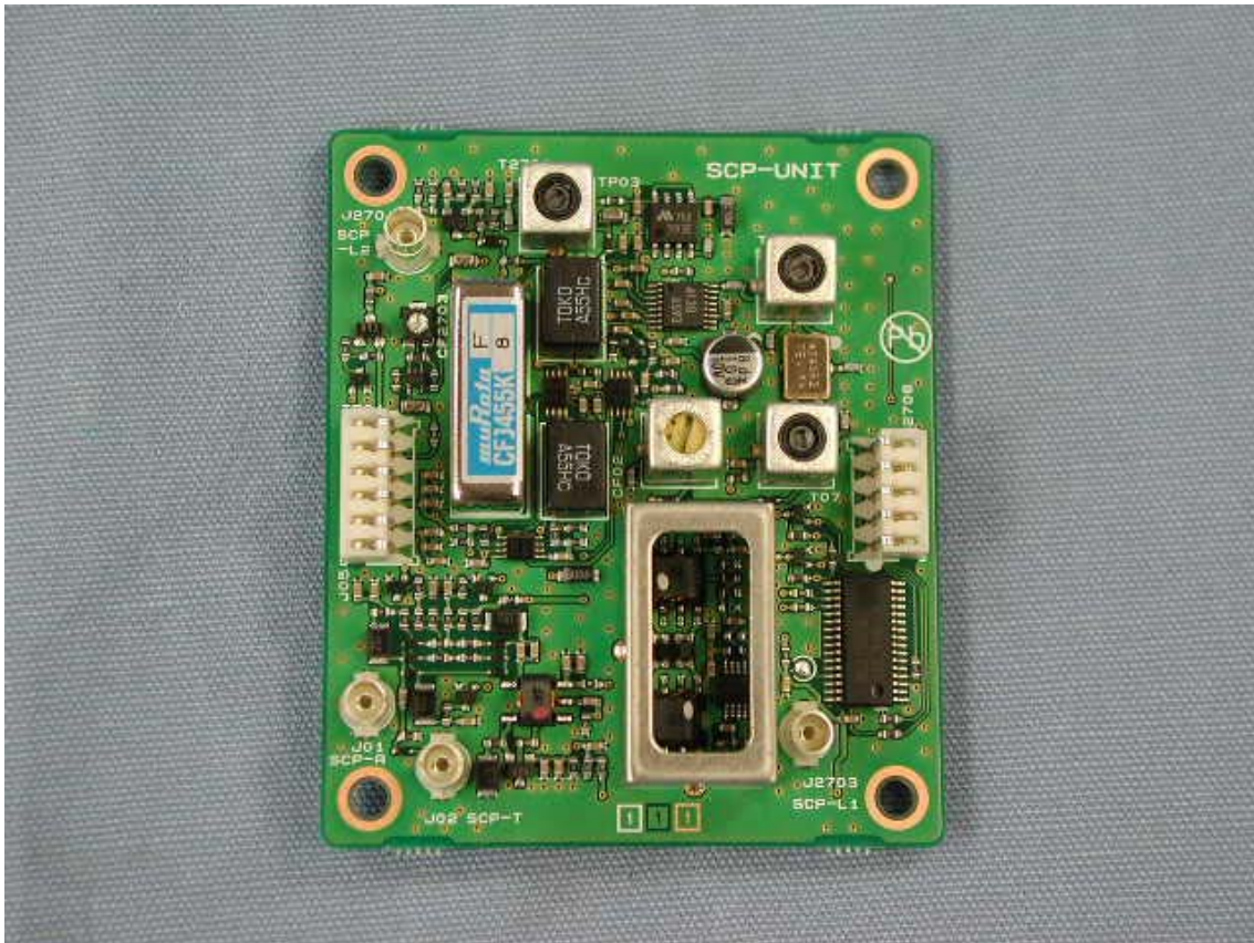
Side-A of SCP -UNIT ON TRX-UNIT
