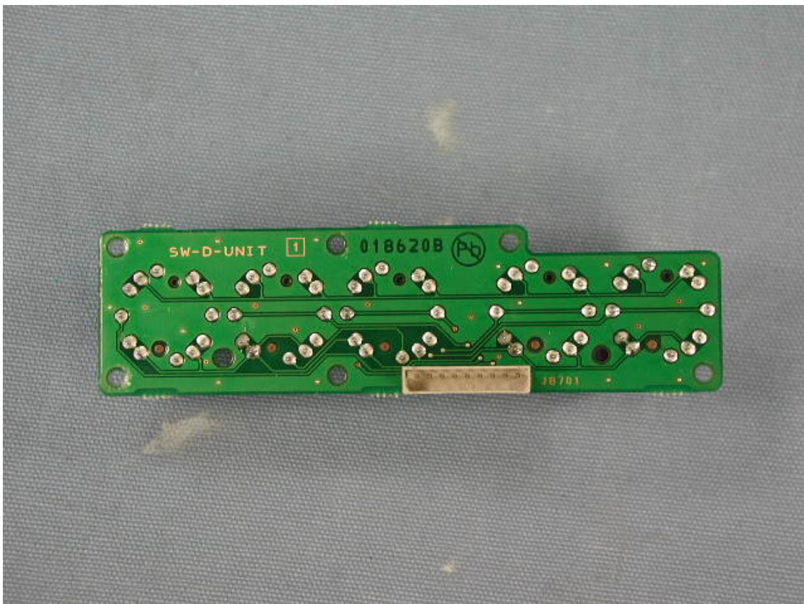
Side-B of SW-D-UNIT
