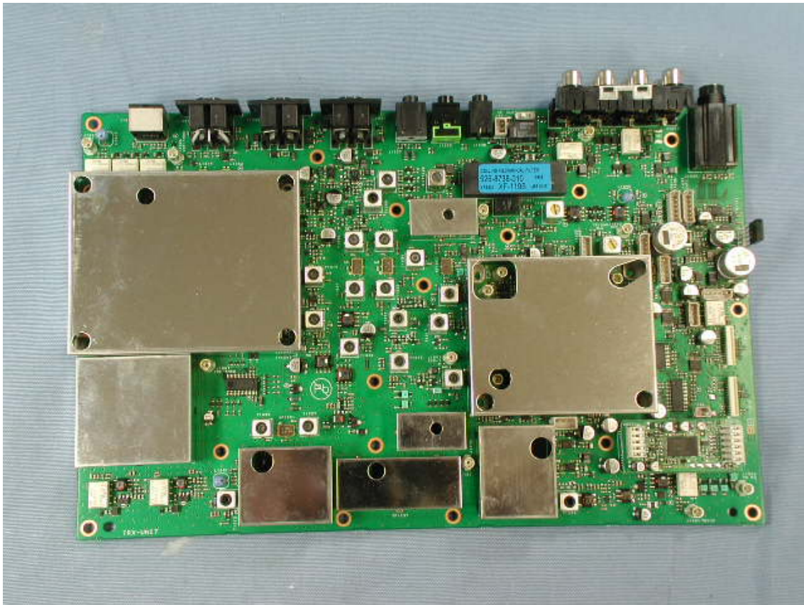
Side-A of TRX-UNIT with shield cases
