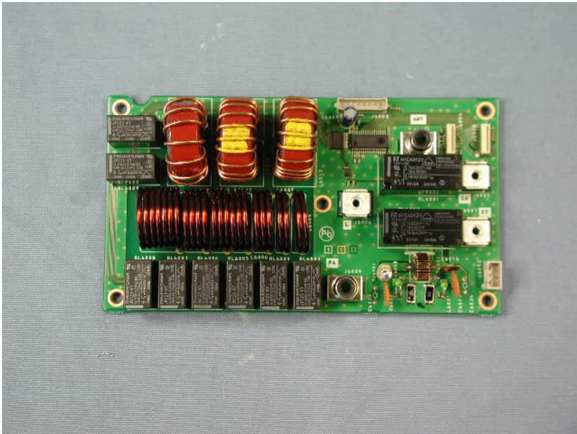
Side-A of TUNER-UNIT
