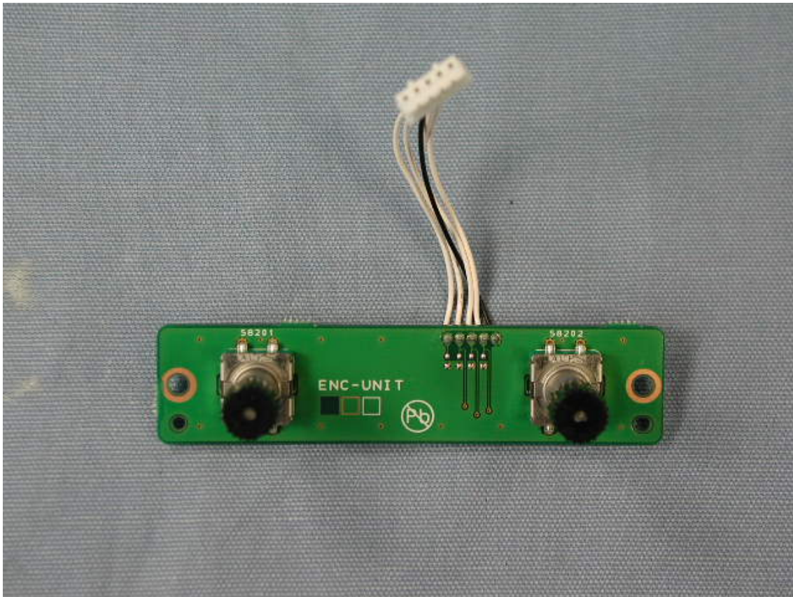
Side-A of ENC-UNIT
