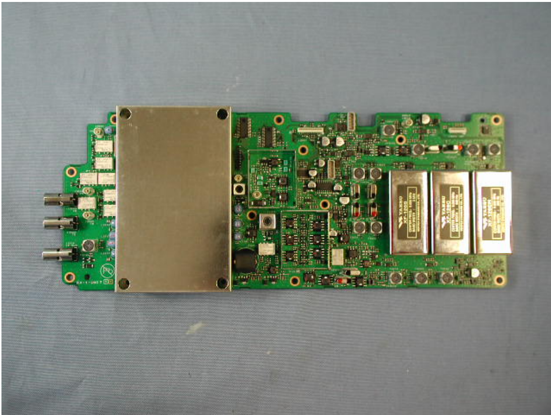
Side-A of RX-UNIT with shield cases
