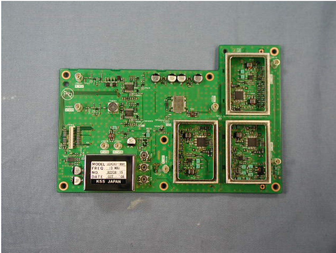
Side-A of LOCAL-UNIT without shield case
