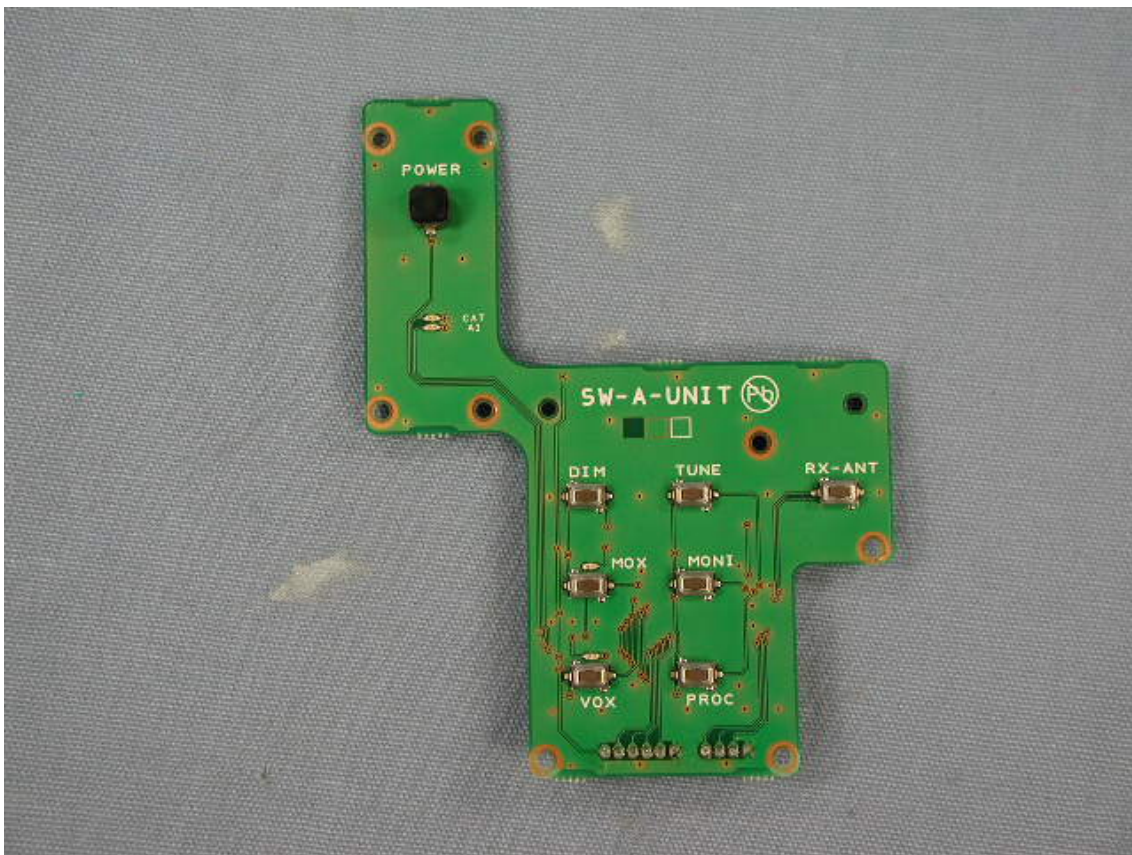
Side-A of SW-A-UNIT
