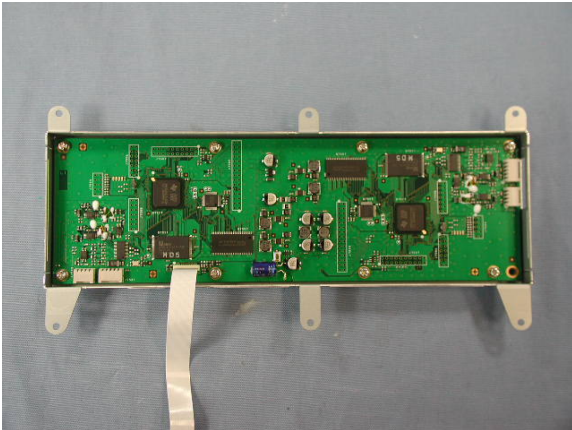
Side- A of DSP-UNIT Without shield Cover
