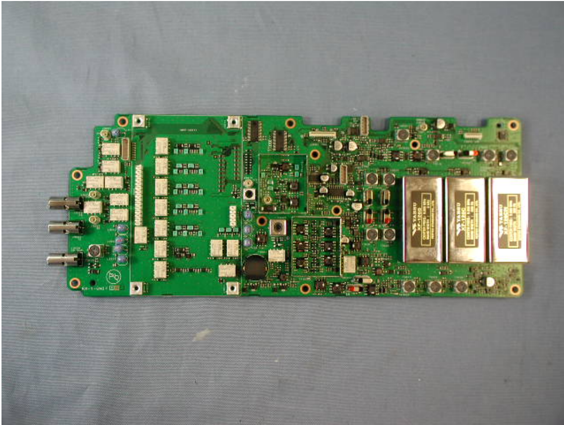
Side-A of RX-UNIT without BPF-UNIT
