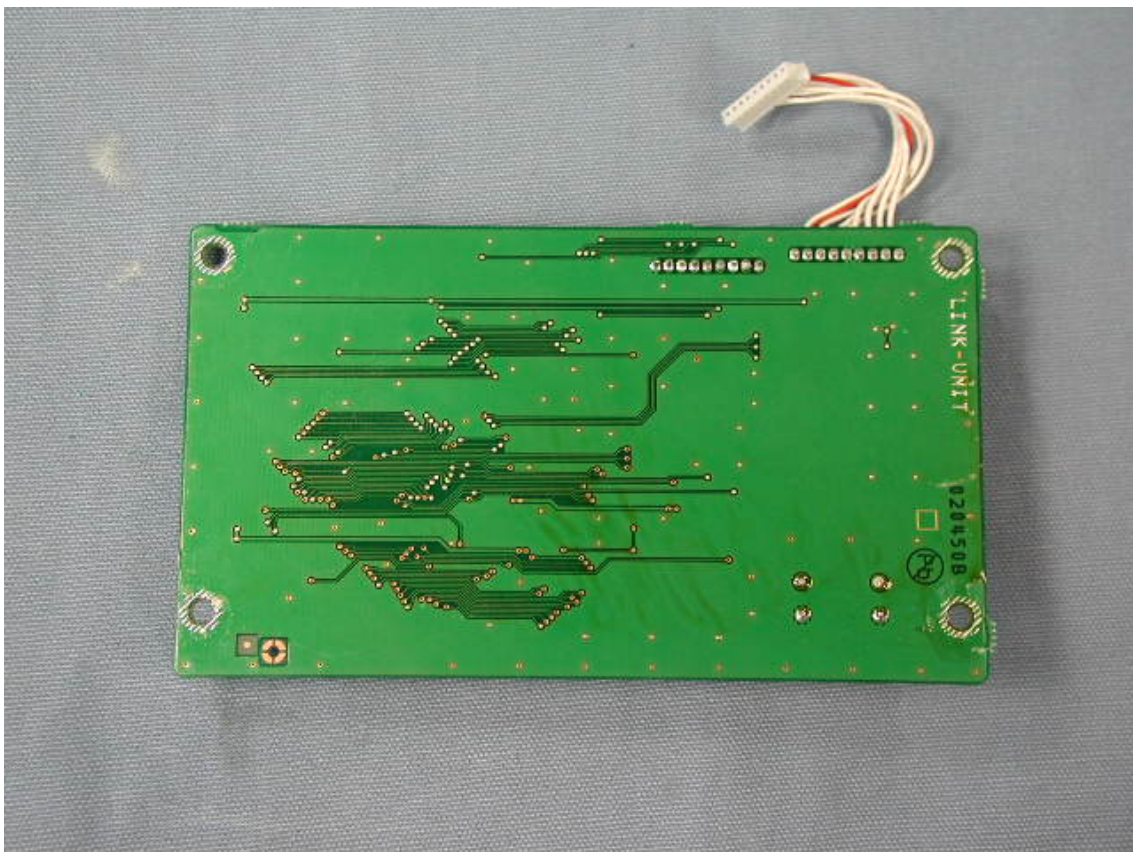
Side-B of LINK-UNIT
