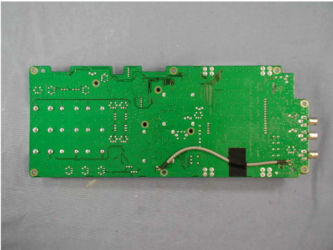
Side-B of RX-UNIT
