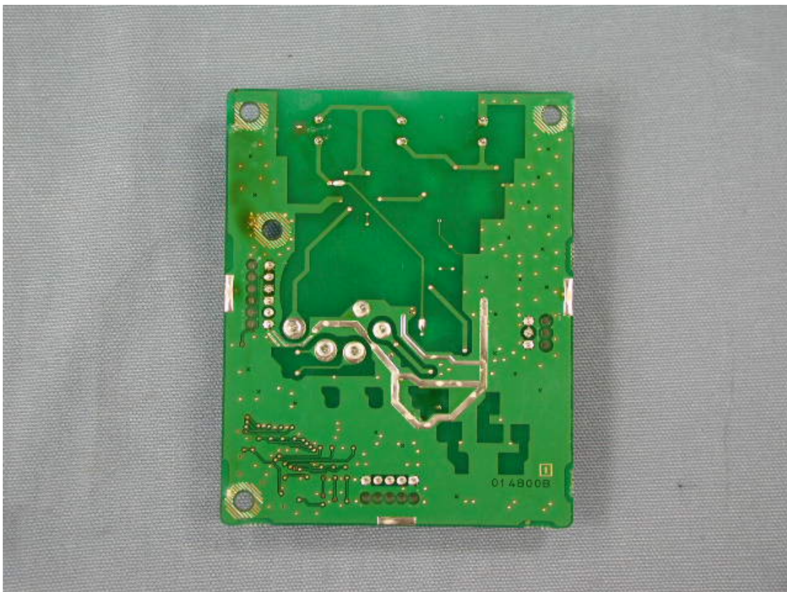
Side-B of VRF-UNIT on TRX -UNIT
