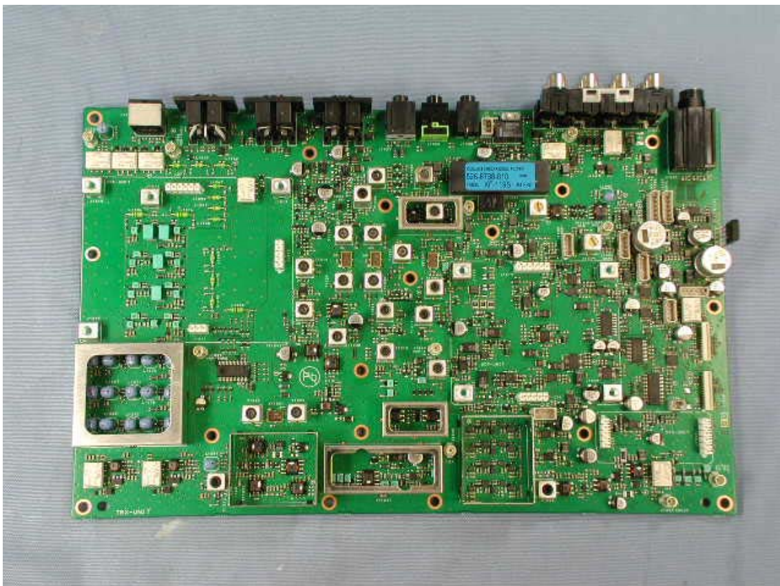
Side-A of TRX-UNIT without VRF / SCP / FM-UNIT
