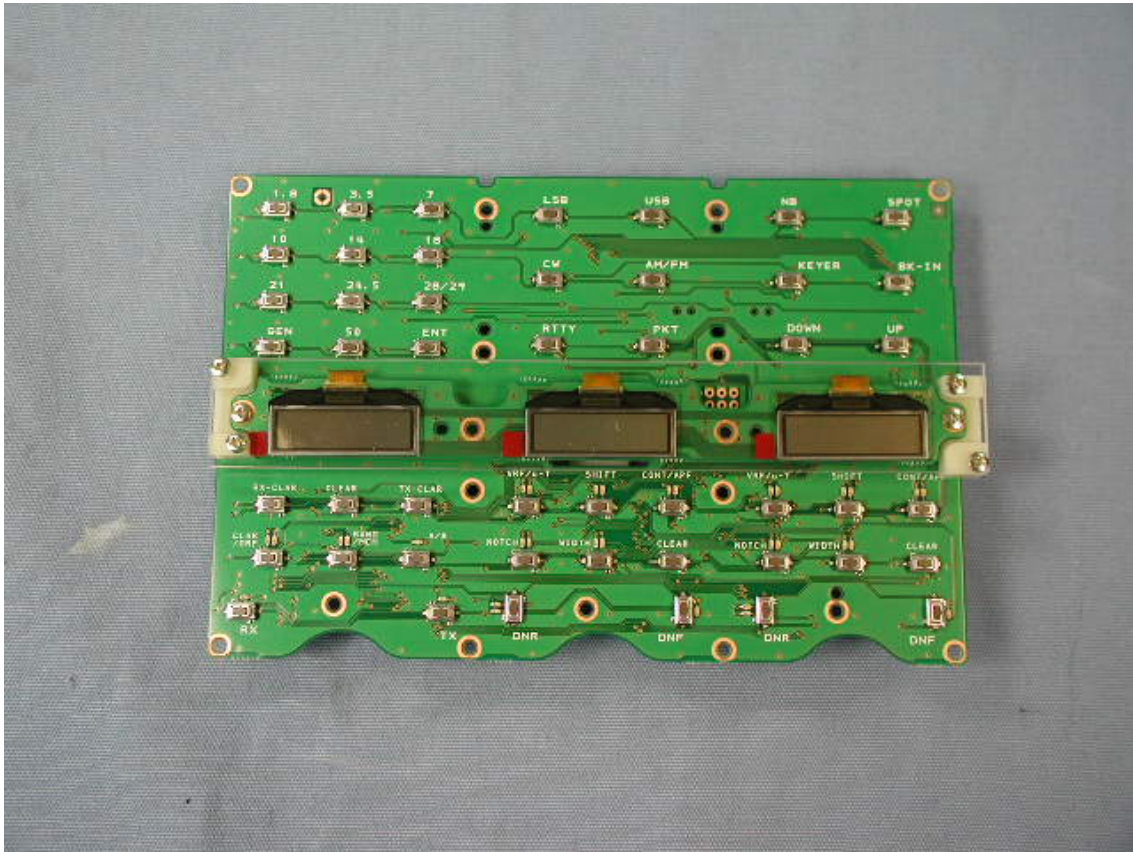
Side-A of SW-B-UNIT With UEL-UNIT
