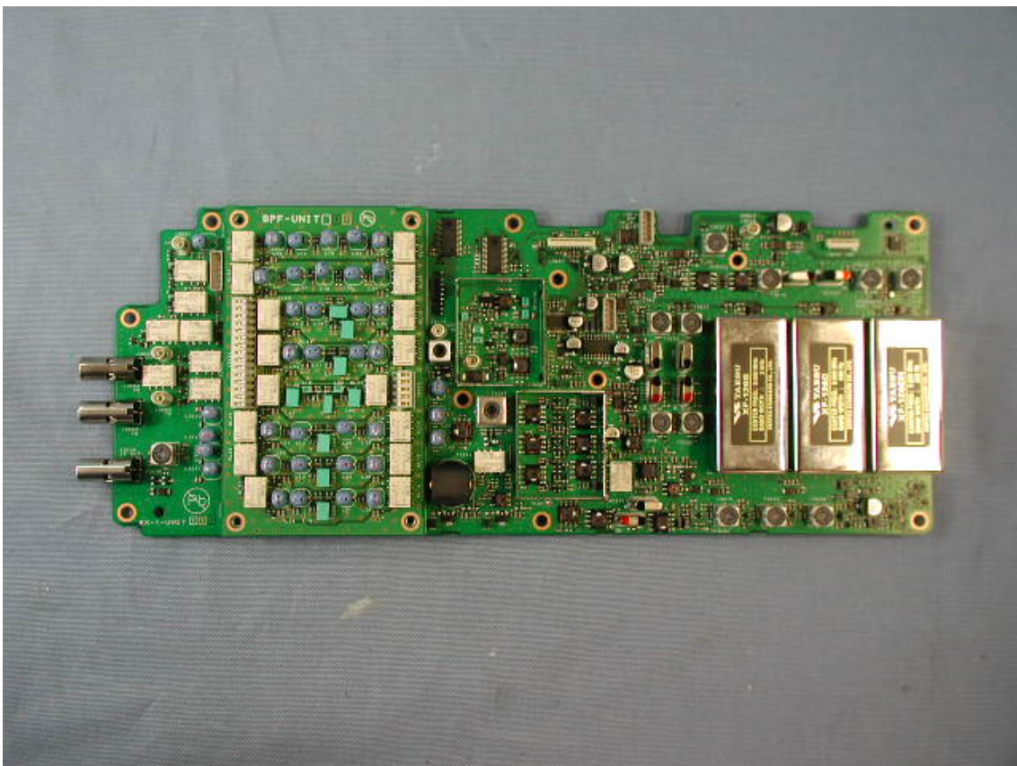
Side-A of RX-UNIT without shield cases
