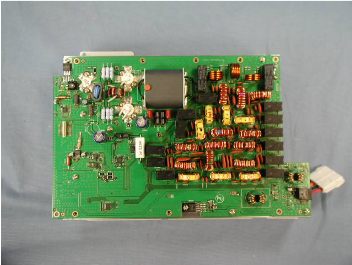
Side-A of PA-B-UNIT
