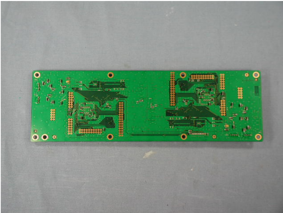
Side-B of DSP-UNIT
