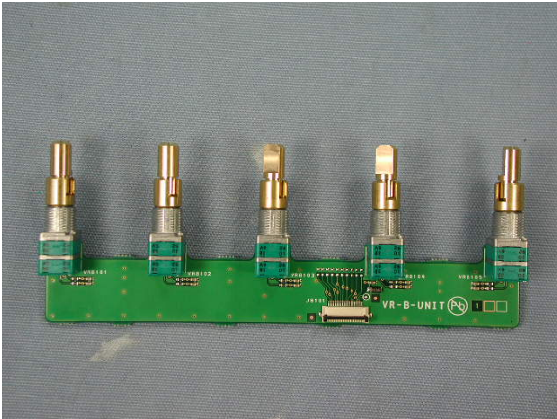
Side-A of VR-B-UNIT
