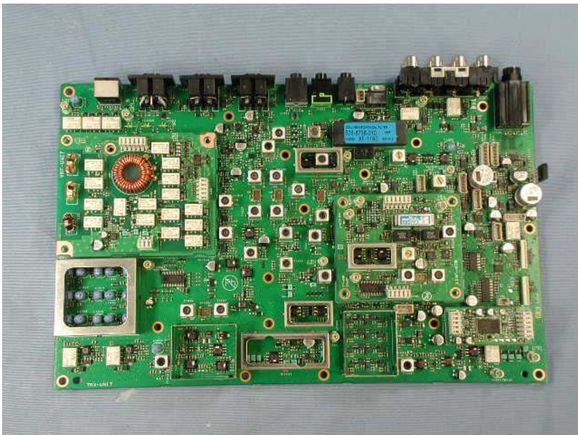
Side-A of TRX-UNIT without shield cases
