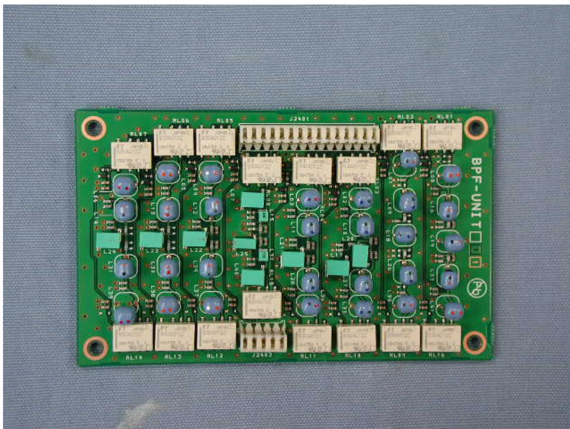
Side-A of BPF-UNIT ON RX-UNIT
