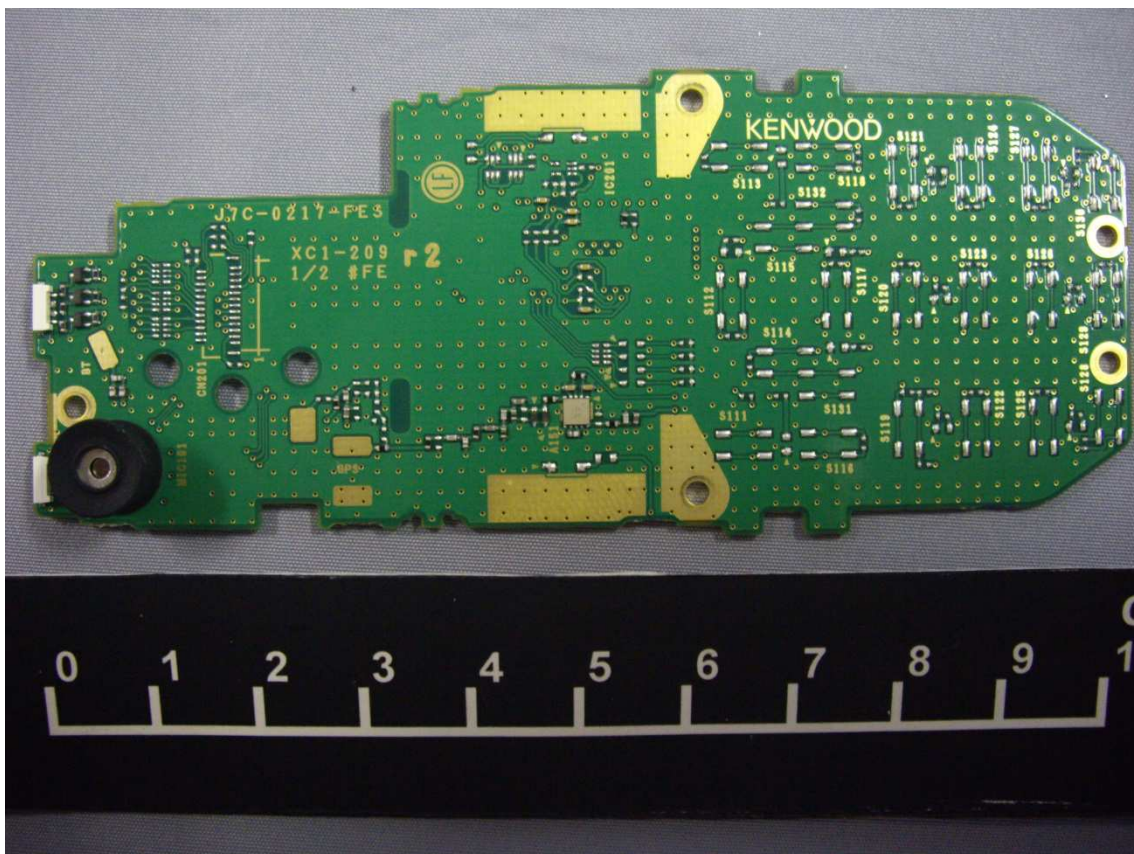
DISPLAY Unit of NX-3320-K (Top)
