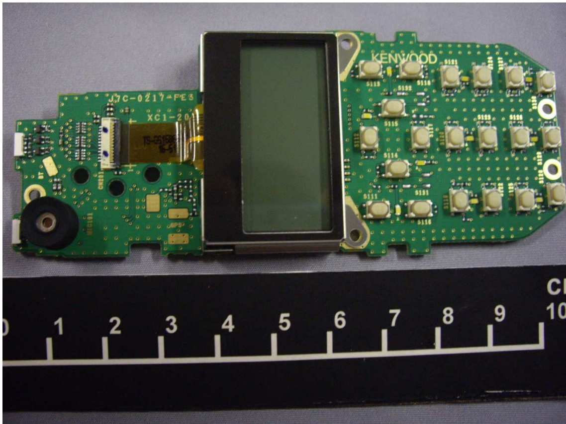
DISPLAY Unit of NX-3320-K3 (Top)
