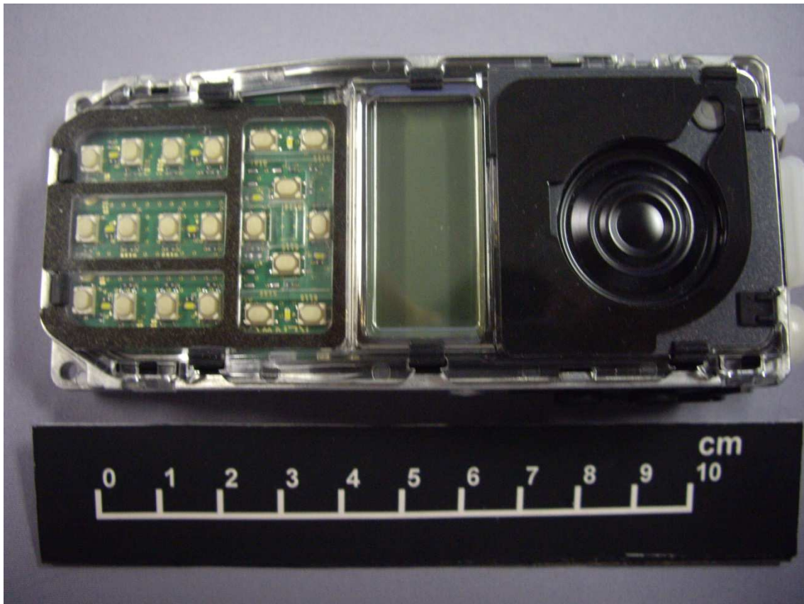
Top Internal View of NX-3320-K3
