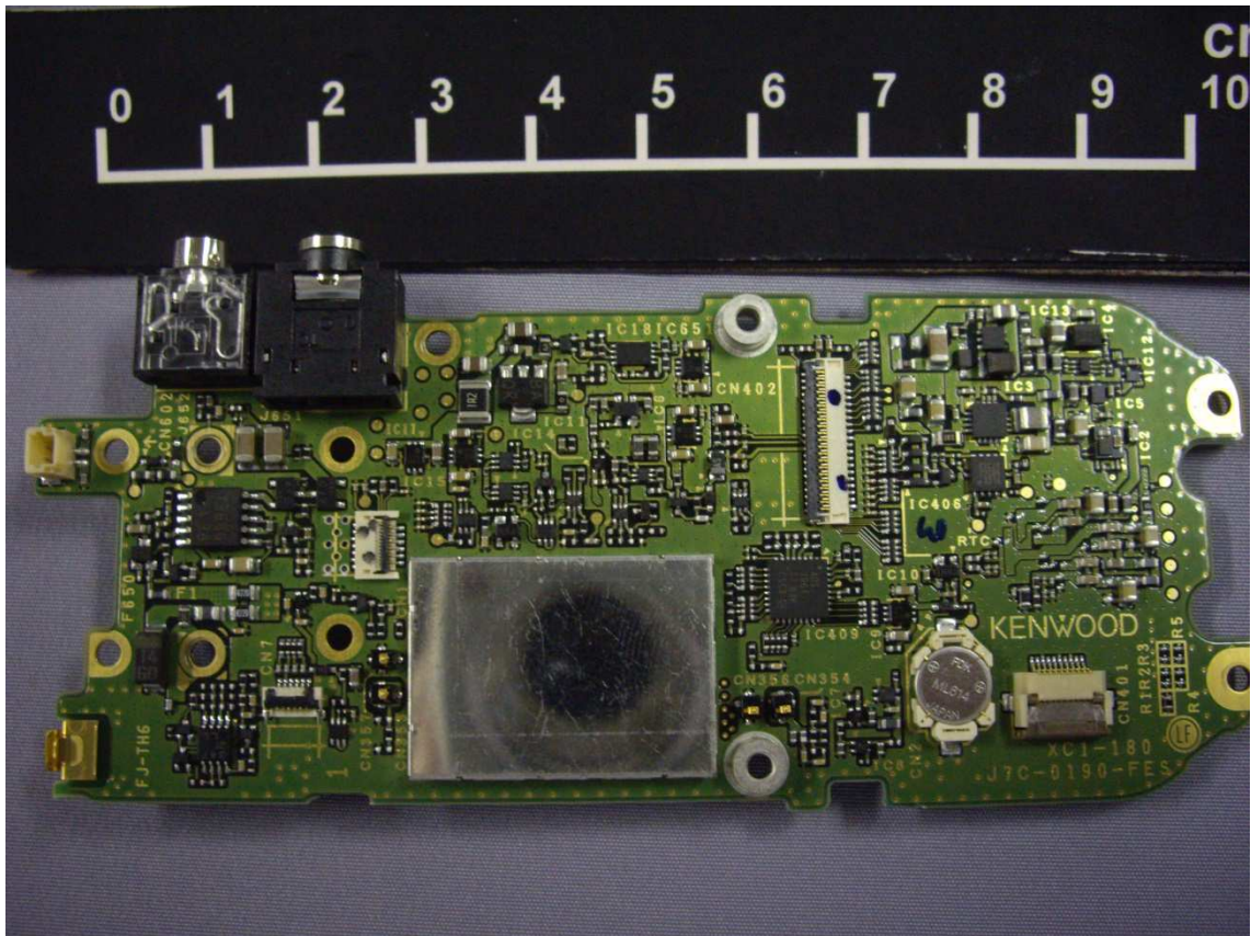
TX-RX Unit of NX-3320-K_K2_K3 (Top)
