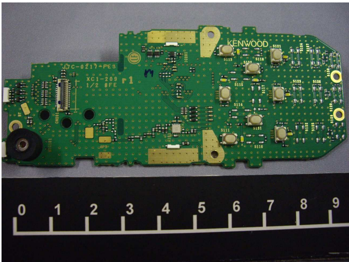
DISPLAY Unit without LCD of NX-3320-K2 (Top)
