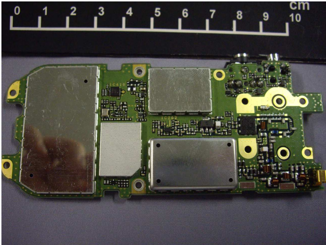
TX-RX Unit of NX-3320-K_K2_K3 (Bottom)
