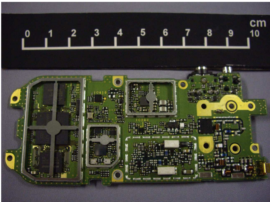
TX-RX Unit of NX-3320-K_K2_K3 without shield case (Bottom)
