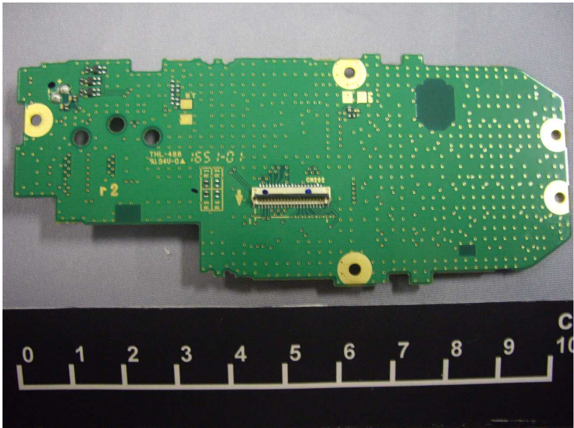
DISPLAY Unit of NX-3320-K3 (Bottom)
