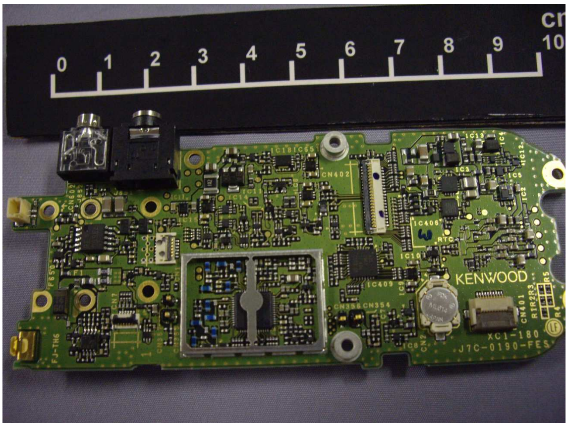
TX-RX Unit of NX-3320-K_K2_K3 without shield case (Top)
