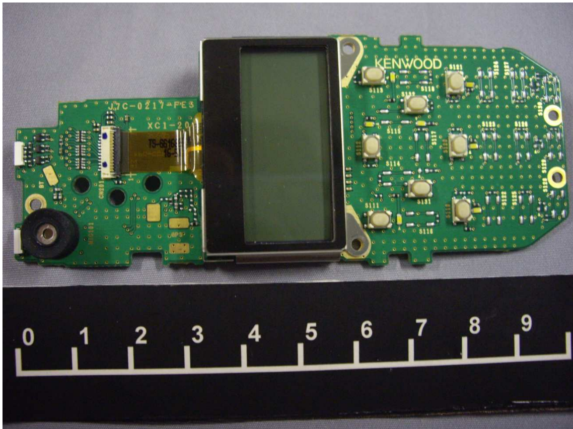
DISPLAY Unit of NX-3320-K2 (Top)
