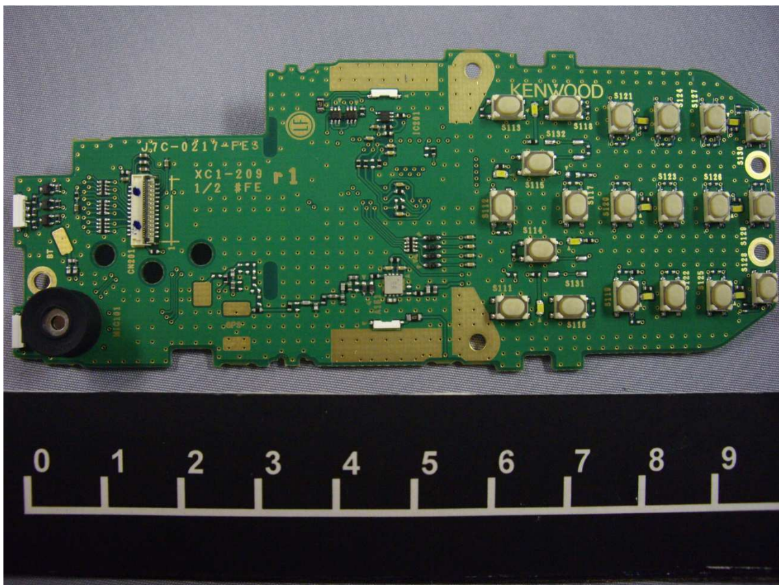
DISPLAY Unit without LCD of NX-3320-K3 (Top)
