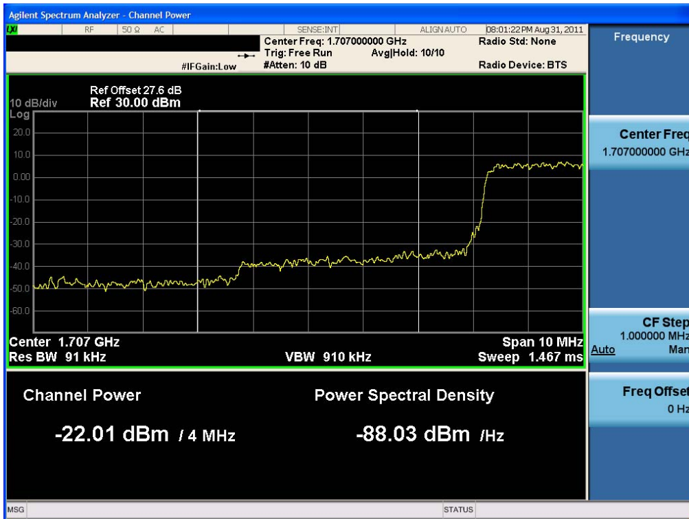
Extended Band Edge Plot (5 MHz BW, QPSK, AWS Band – Low Channel)
