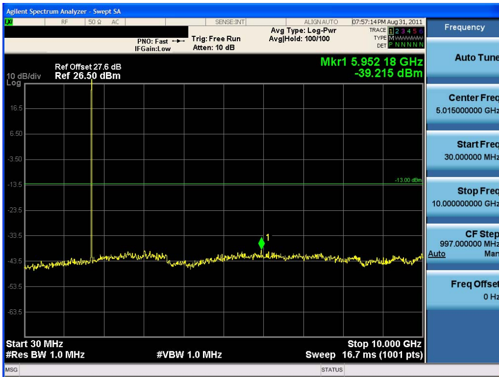
Conducted Spurious Plot (5 MHz BW, 16-QAM, Band 4 – Low Channel)
