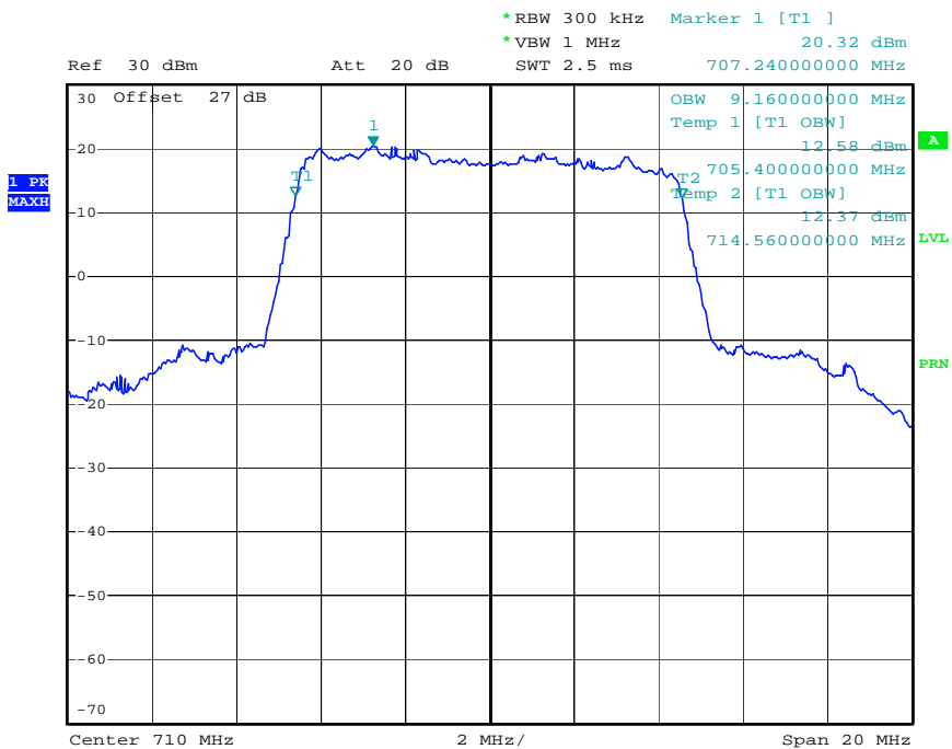
Occupied Bandwidth Plot (10MHz BW, QPSK, Band 17)
