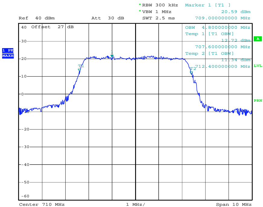
Occupied Bandwidth Plot (5 MHz BW, QPSK, Band 17)
