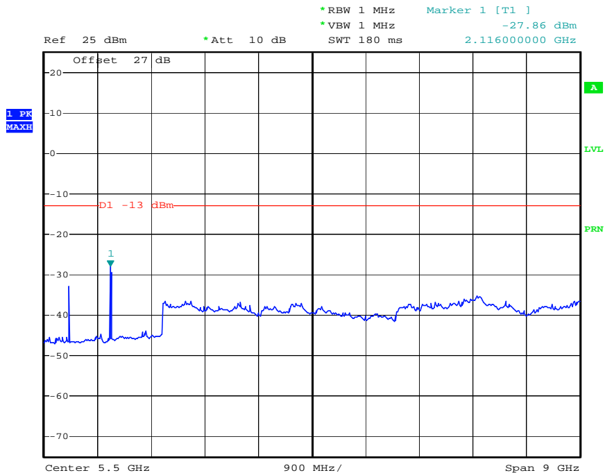
Conducted Spurious Plot (10 MHz BW, QPSK, Band 17 -710 MHz)
