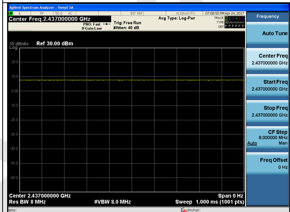
Test plot of Duty Cycle for 802.11n(HT40)
