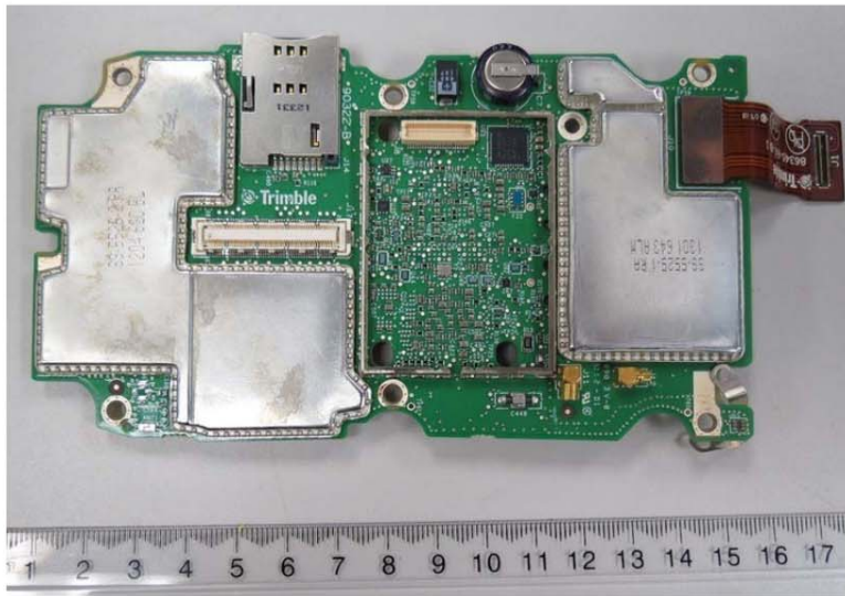
Main Board top + cellular modem removed
