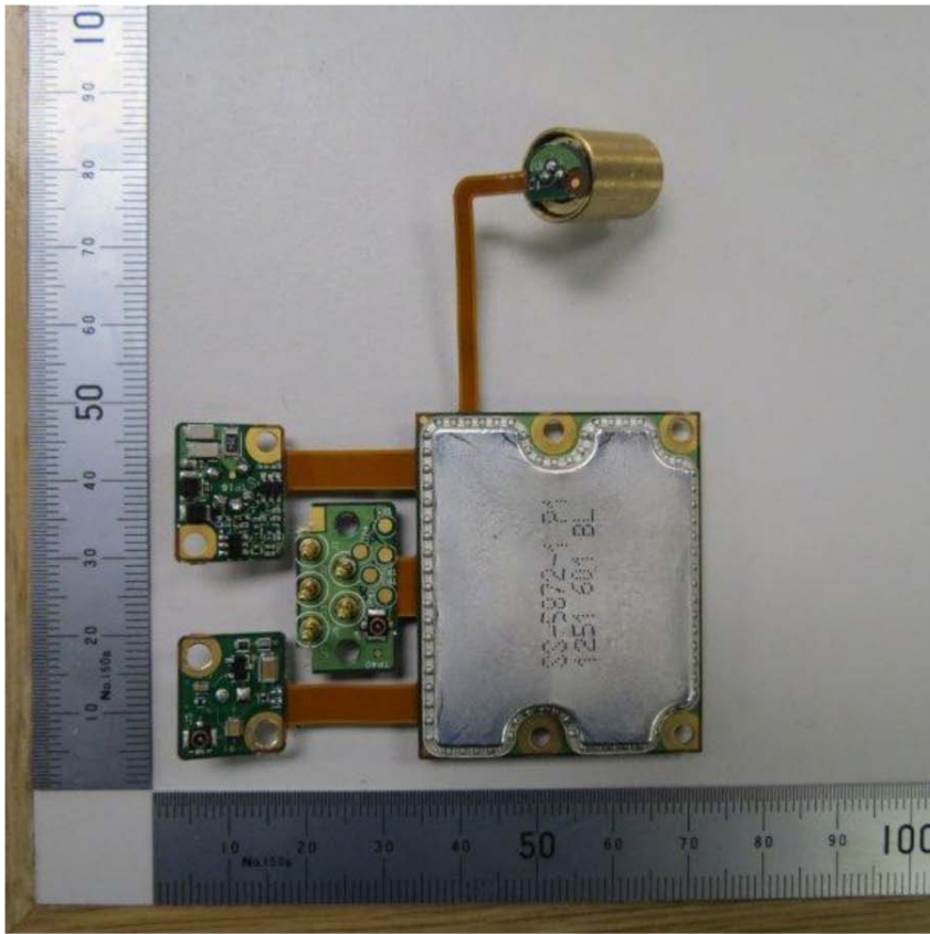
Printed circuit board assemblies, top view, GORE®shield fitted
