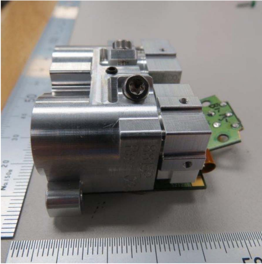
Optical bench, side view
