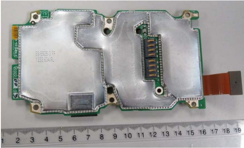
Main Board bottom
