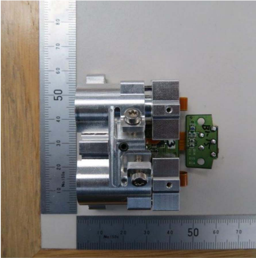
Optical bench, top view
