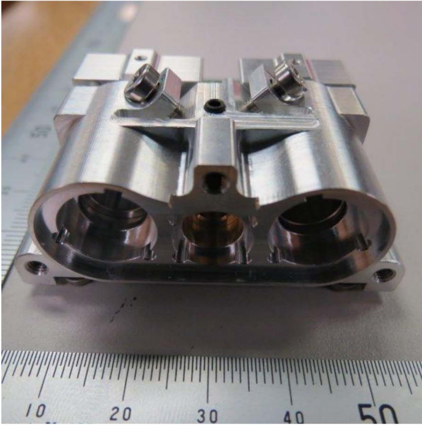
Optical bench, front view
