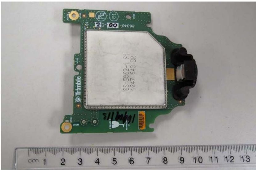
Sensor Board top
