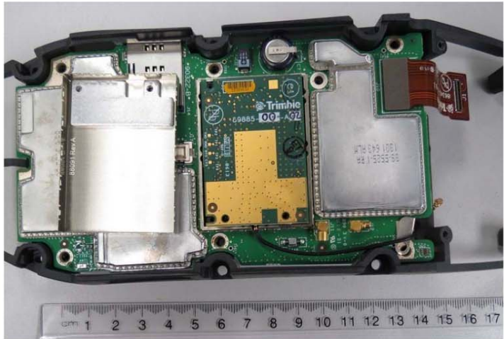
Main Board top + cellular modem can removed
