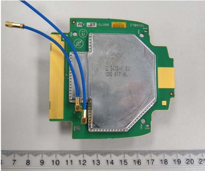
Low Noise Amplifier (LNA) Board bottom
