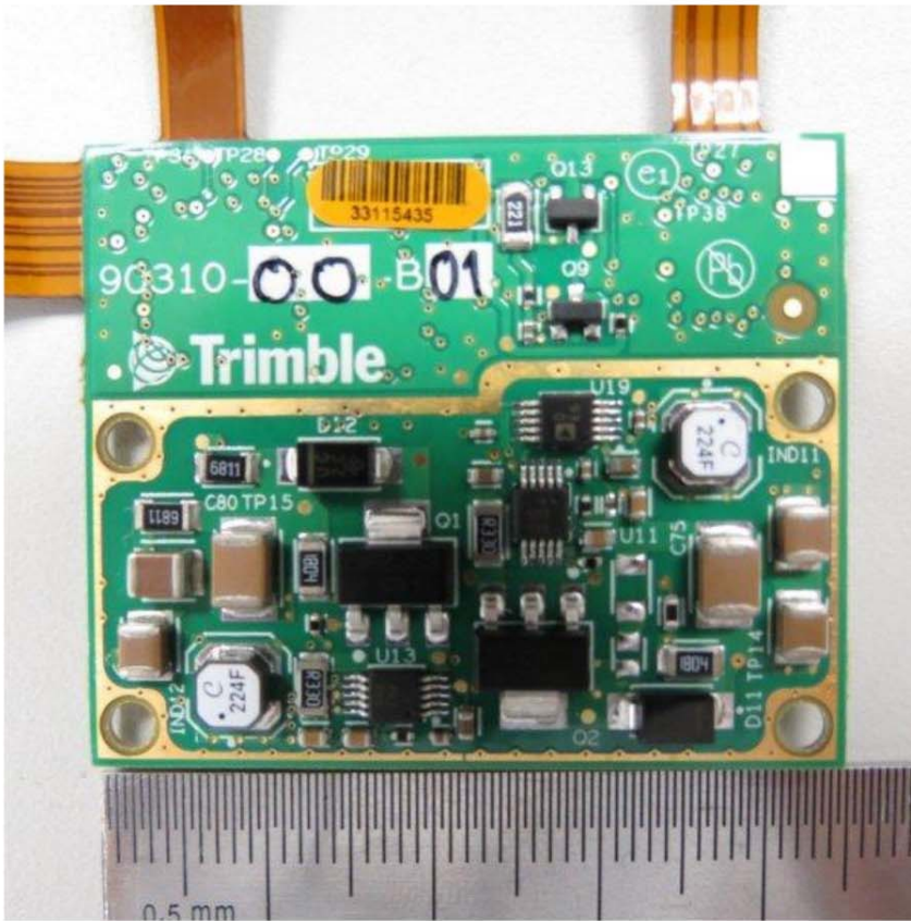
Main board, underside detail view, GORE®shield removed
