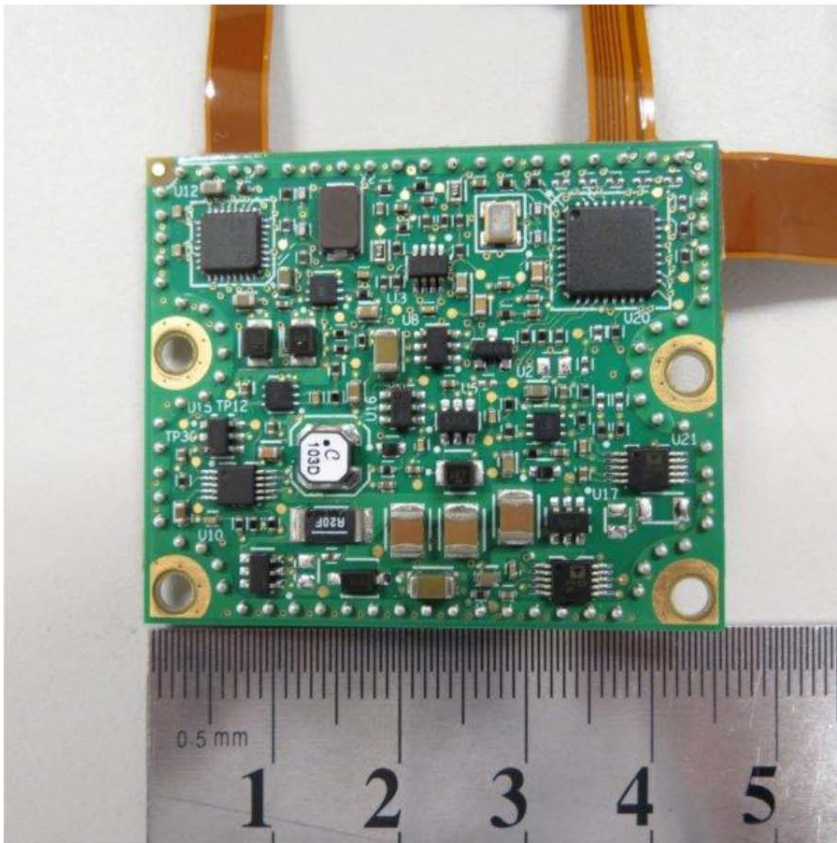
Main board, top detail view, GORE®shield removed
