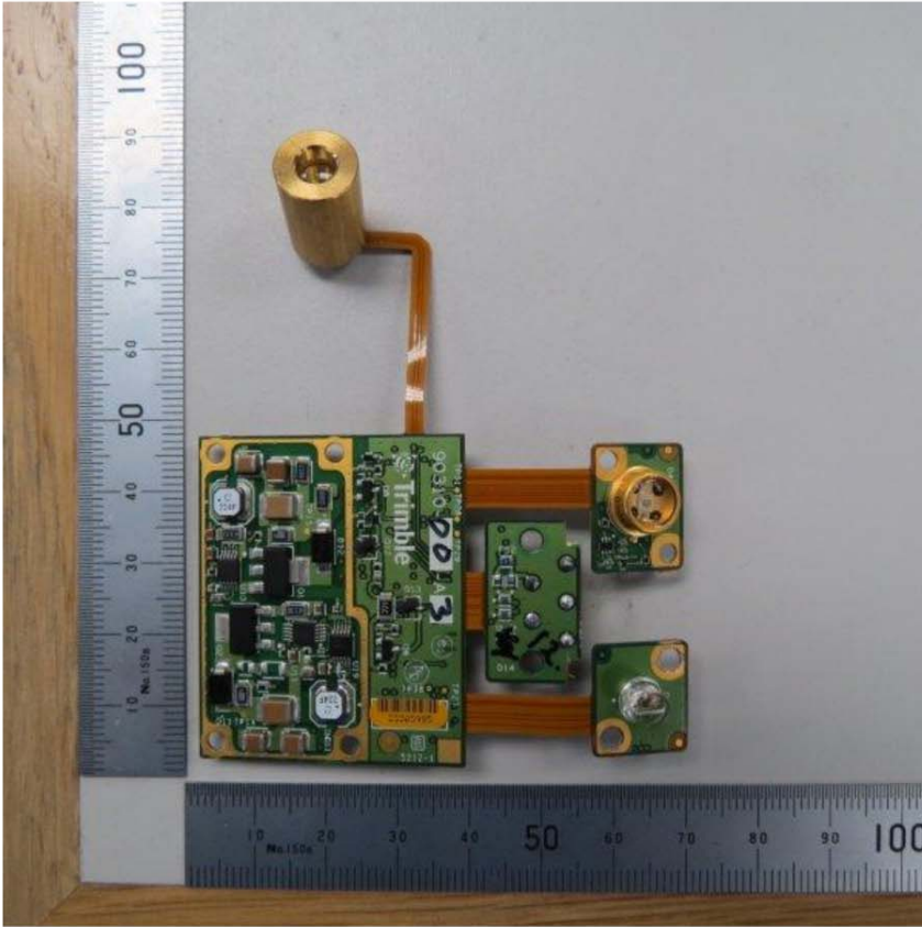
Printed circuit board assembly underside, showing optics components
