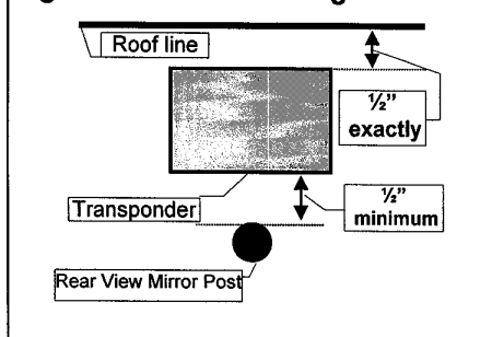
Fig.-2 Preferred Mounting Location
