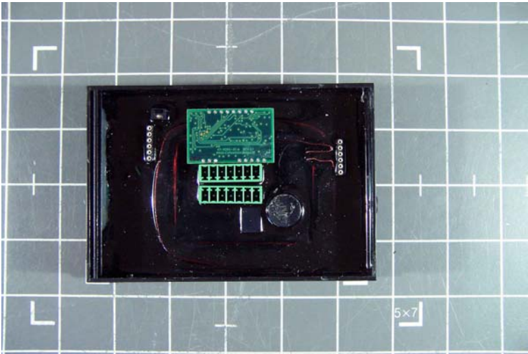
EXTERIOR BACK POTTED 6136AxN-A
