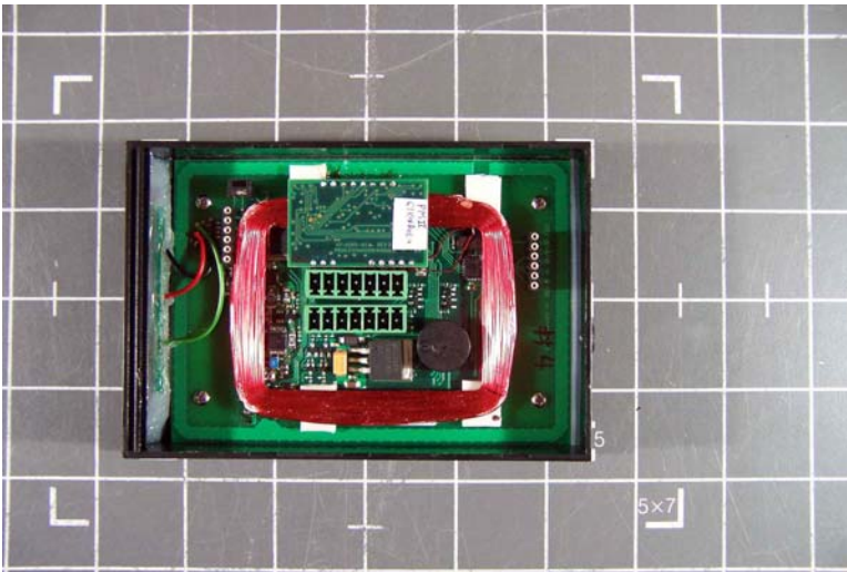
INTERIOR BACK OVERALL
