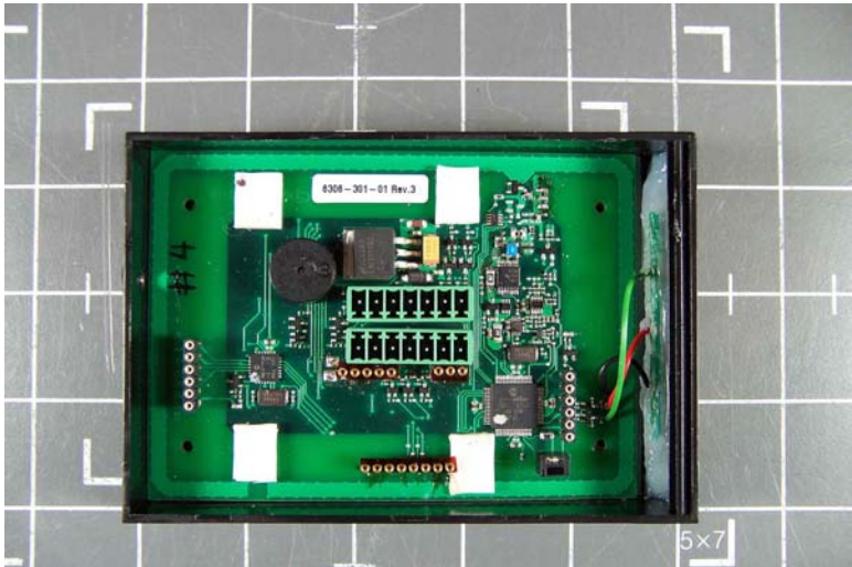
MAIN PCB BACK ALL
