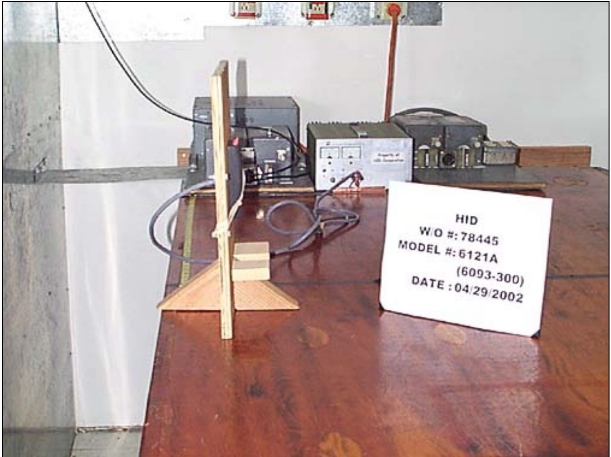
Mains Conducted Emissions - Side View - 6121A
