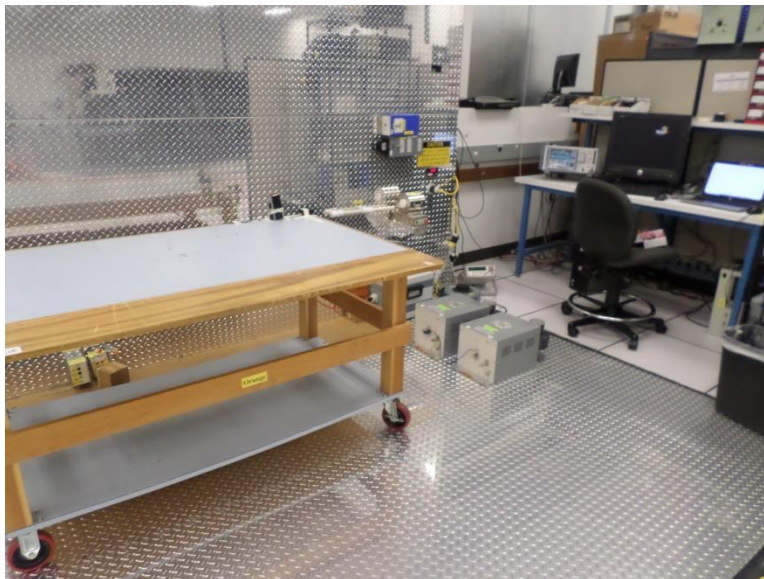
Figure 2: Conducted Emission Limits, Pigtail, Test Setup, Front View
