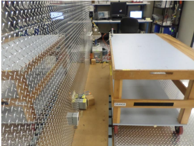
Figure 3: Conducted Emission Limits, Pigtail, Test Setup, Back View
