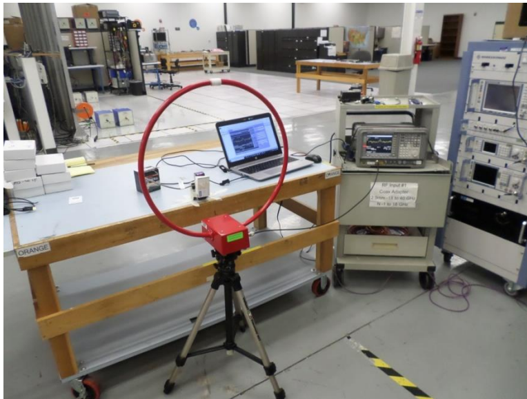
Figure 7: 20 dB Occupied Bandwidth, Pigtail, Test Setup
