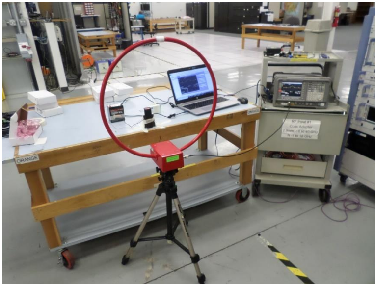
Figure 8: 20 dB Occupied Bandwidth, Terminal, Test Setup
