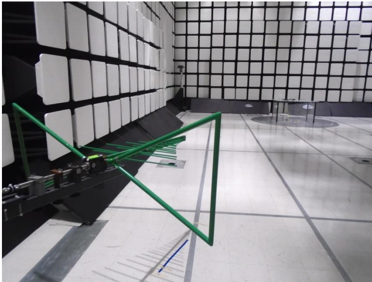
Figure 10: Radiated Spurious Emissions, 30 MHz – 1000 MHz, Test Setup
