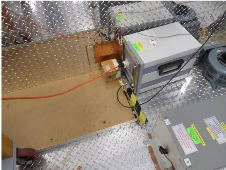
Figure 1: Conducted Emission Limits, Pigtail, Test Setup, LISN View
