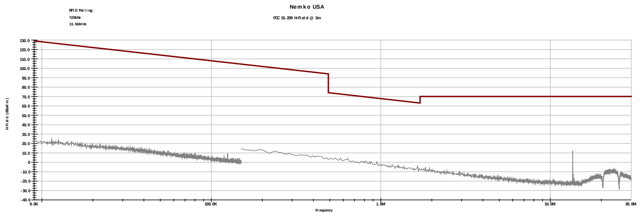
Plot 8.3-1: Radiated emissions - Loop Antenna 90 degree
