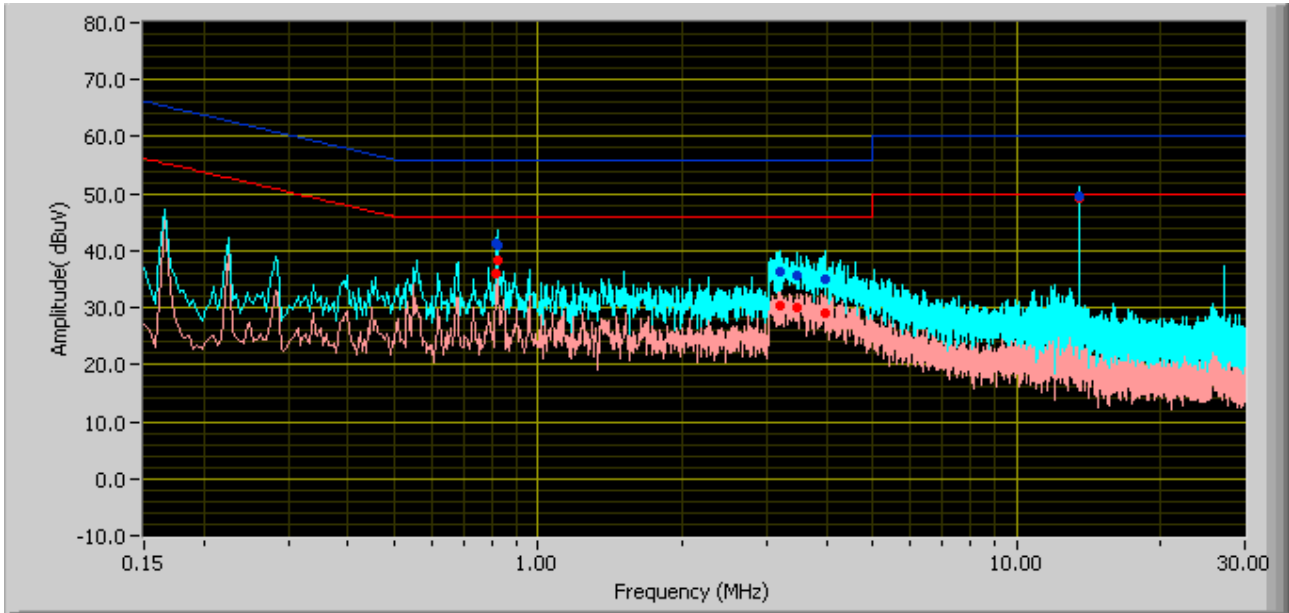
120VAC,60Hz, Neutral Line
