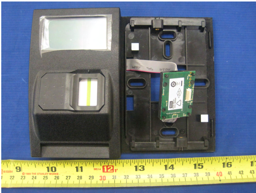
EUT RFID Reader Remove Top View
