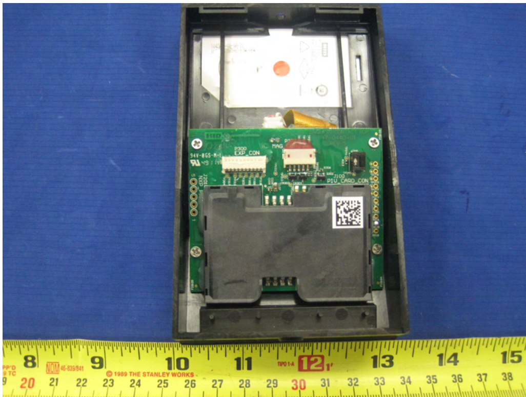
EUT Remove from Connector View
