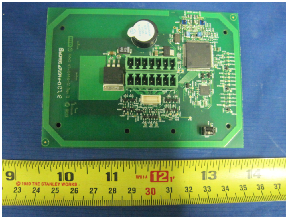
Reader Main Board Bottom View
