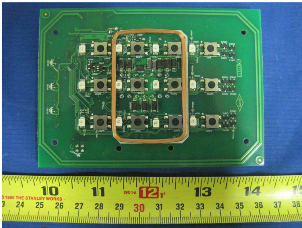
Reader Main Board Top View
