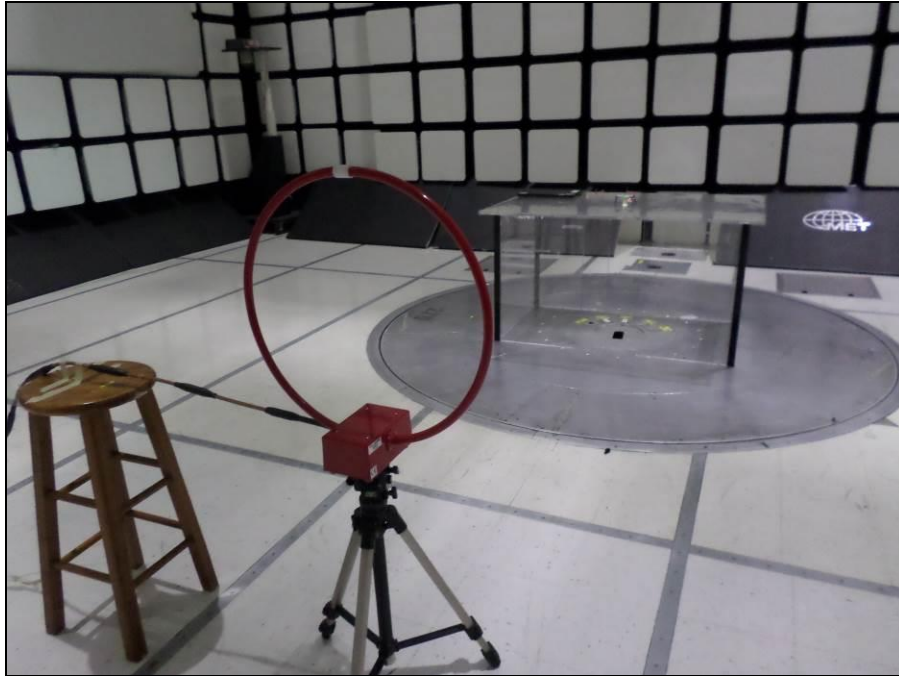
Photograph 3. Radiated Emissions, 0.009 MHz – 1.250 MHz, Antenna View
