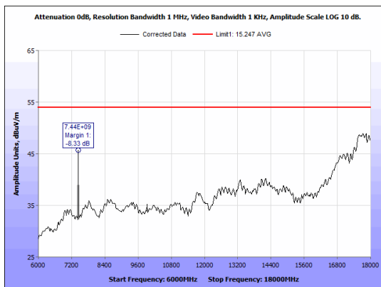
Figure 44: Radiated Emissions, BLE High Channel, 6GHz - 18GHz, Average, Antenna 2
