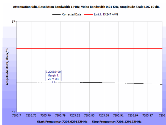
Figure 29: Radiated Emissions, BLE Low Channel, Average, 7.2 GHz, emission, Antenna 2
