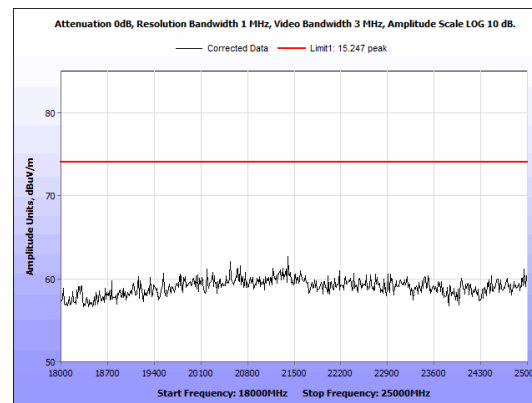
Figure 16: Radiated Emissions, BLE Low Channel, 18GHz - 25GHz, Peak, Antenna 1
