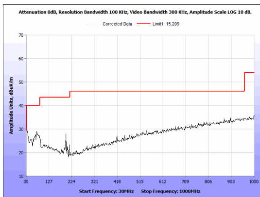
Figure 42: Radiated Emissions, BLE High Channel, 30 MHz - 1 GHz Antenna 2
