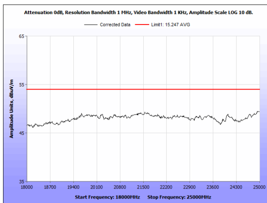
Figure 45: Radiated Emissions, BLE High Channel, 18GHz - 25GHz, Average, Antenna 2
