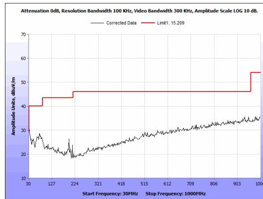
Figure 35: Radiated Emissions, BLE Mid Channel, 30 MHz - 1 GHz Antenna 2
