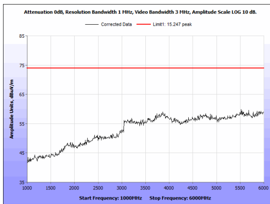
Figure 46: Radiated Emissions, BLE High Channel, 1GHz - 6 GHz, Peak, Antenna 2
