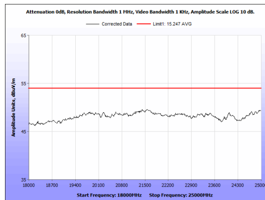
Figure 19: Radiated Emissions, BLE Mid Channel, 18GHz - 25GHz, Average, Antenna 1
