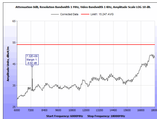
Figure 37: Radiated Emissions, BLE Mid Channel, 6GHz - 18GHz, Average, Antenna 2
