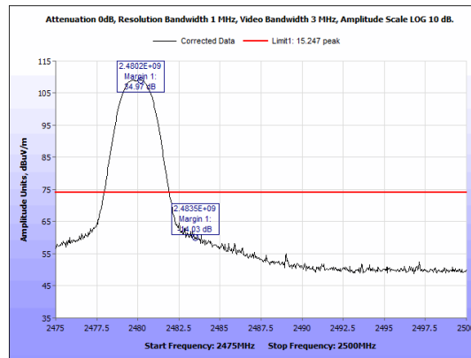
Figure 55: Radiated Emissions, BLE High Channel, Band Edge, Peak, Antenna 2
