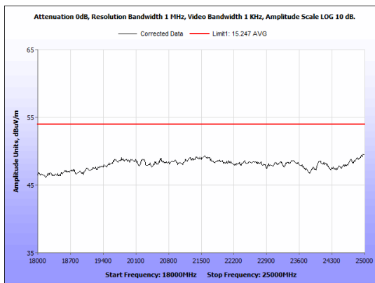
Figure 31: Radiated Emissions, BLE Low Channel 18GHz - 25GHz, Average, Antenna 2
