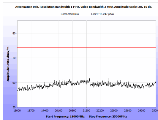
Figure 48: Radiated Emissions, BLE High Channel, 18GHz - 25GHz, Peak, Antenna 2
