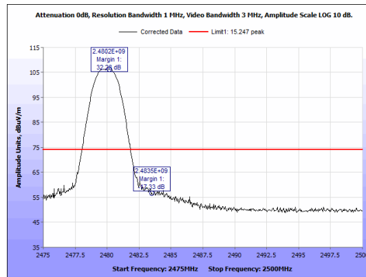
Figure 54: Radiated Emissions, BLE High Channel, Band Edge, Peak, Antenna 1
