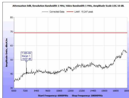
Figure 40: Radiated Emissions, BLE Mid Channel, 6GHz - 18GHz, Peak, Antenna 2
