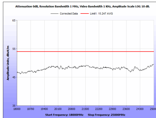
Figure 38: Radiated Emissions, BLE Mid Channel, 18GHz - 25GHz, Average, Antenna 2
