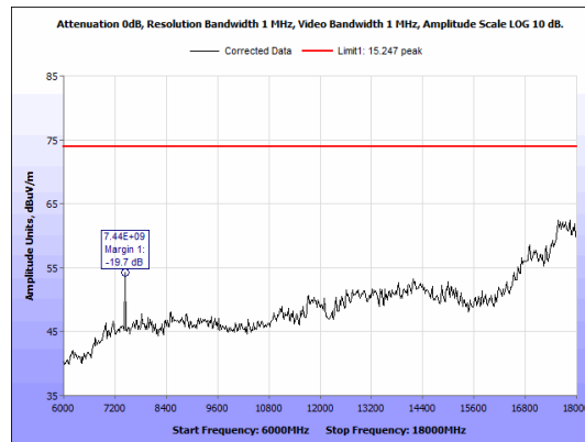
Figure 47: Radiated Emissions, BLE High Channel, 6GHz - 18GHz, Peak, Antenna 2
