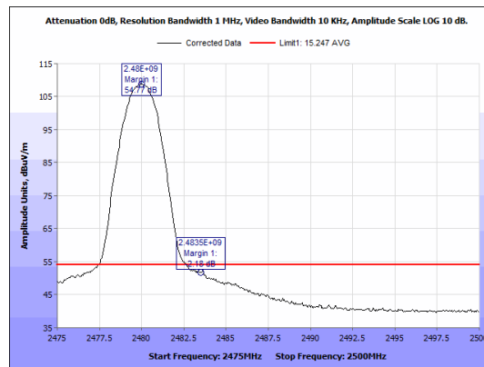
Figure 56: Radiated Emissions, BLE High Channel, Band Edge, Average, Antenna 2
