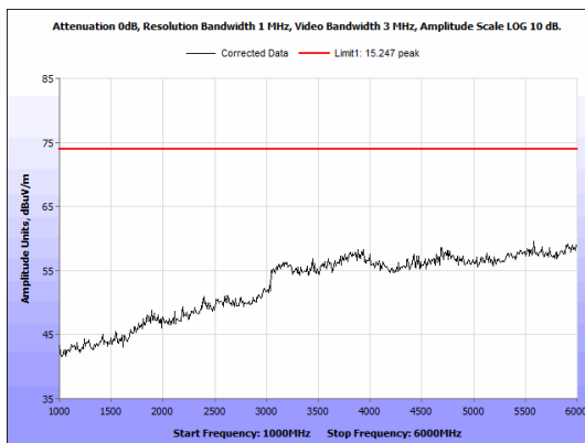
Figure 32: Radiated Emissions, BLE Low Channel 1GHz - 6 GHz, Peak, Antenna 2
