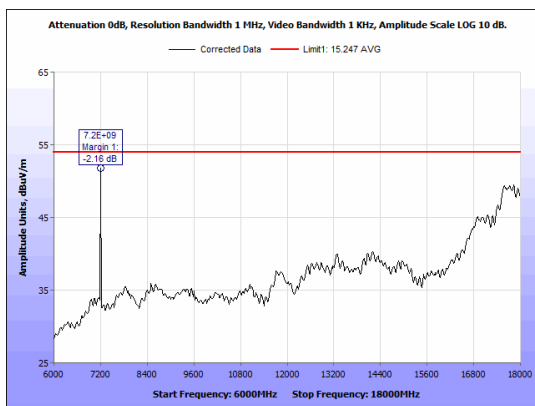
Figure 30: Radiated Emissions, BLE Low Channel 6GHz - 18GHz, Average, Antenna 2
