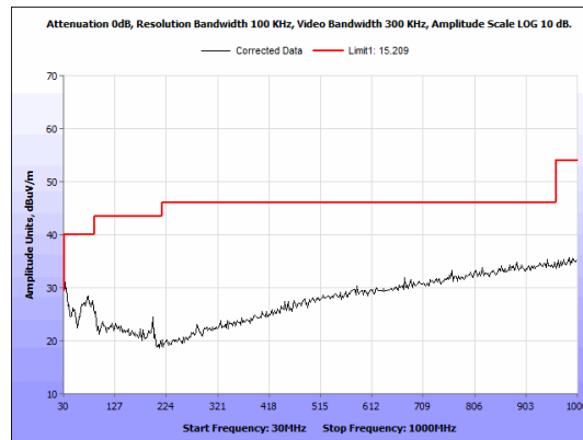
Figure 17: Radiated Emissions, BLE Mid Channel, 30 MHz - 1 GHz Antenna 1
