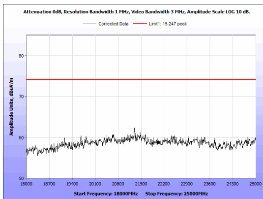
Figure 41: Radiated Emissions, BLE Mid Channel, 18GHz - 25GHz, Peak, Antenna 2
