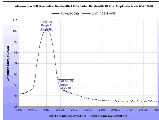
Figure 53: Radiated Emissions, BLE High Channel, Band Edge, Average, Antenna 1
