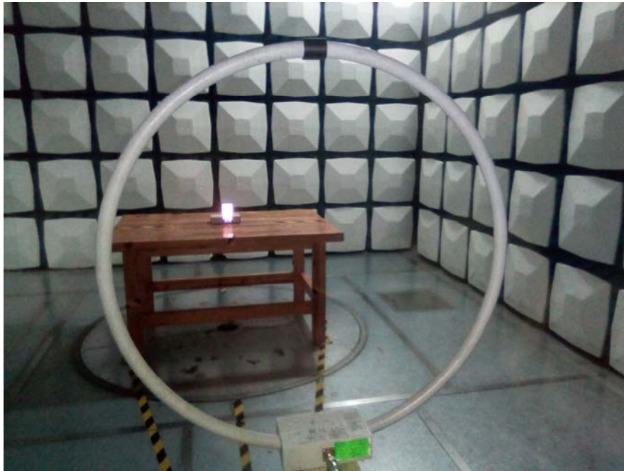
RE 9kHz-30MHz View
