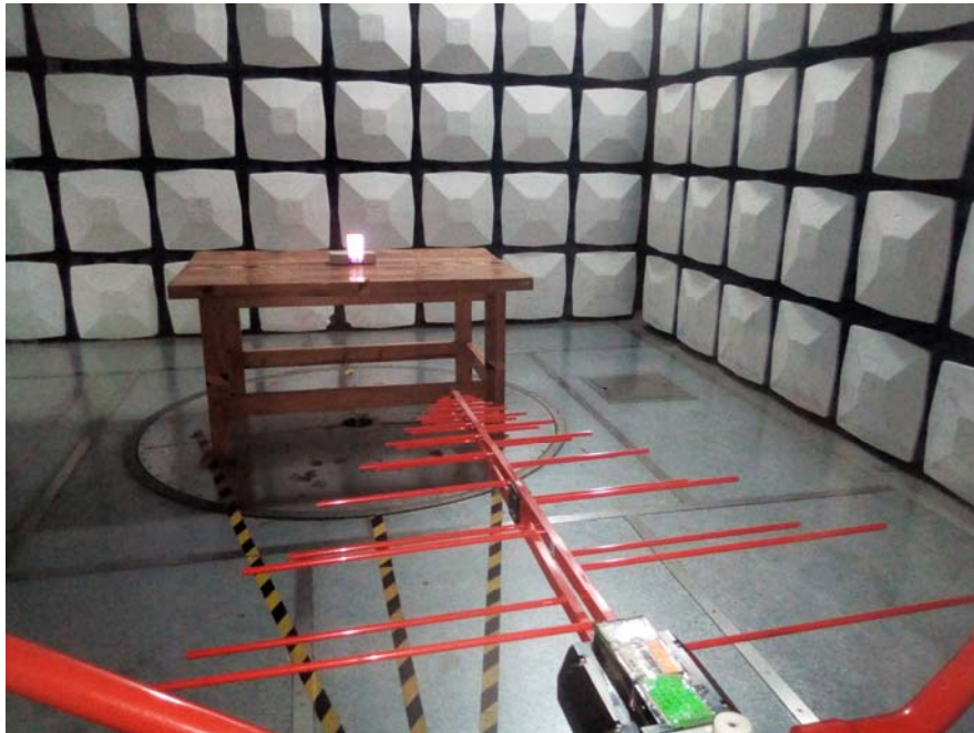
RE 30MHz- 1GHz View
